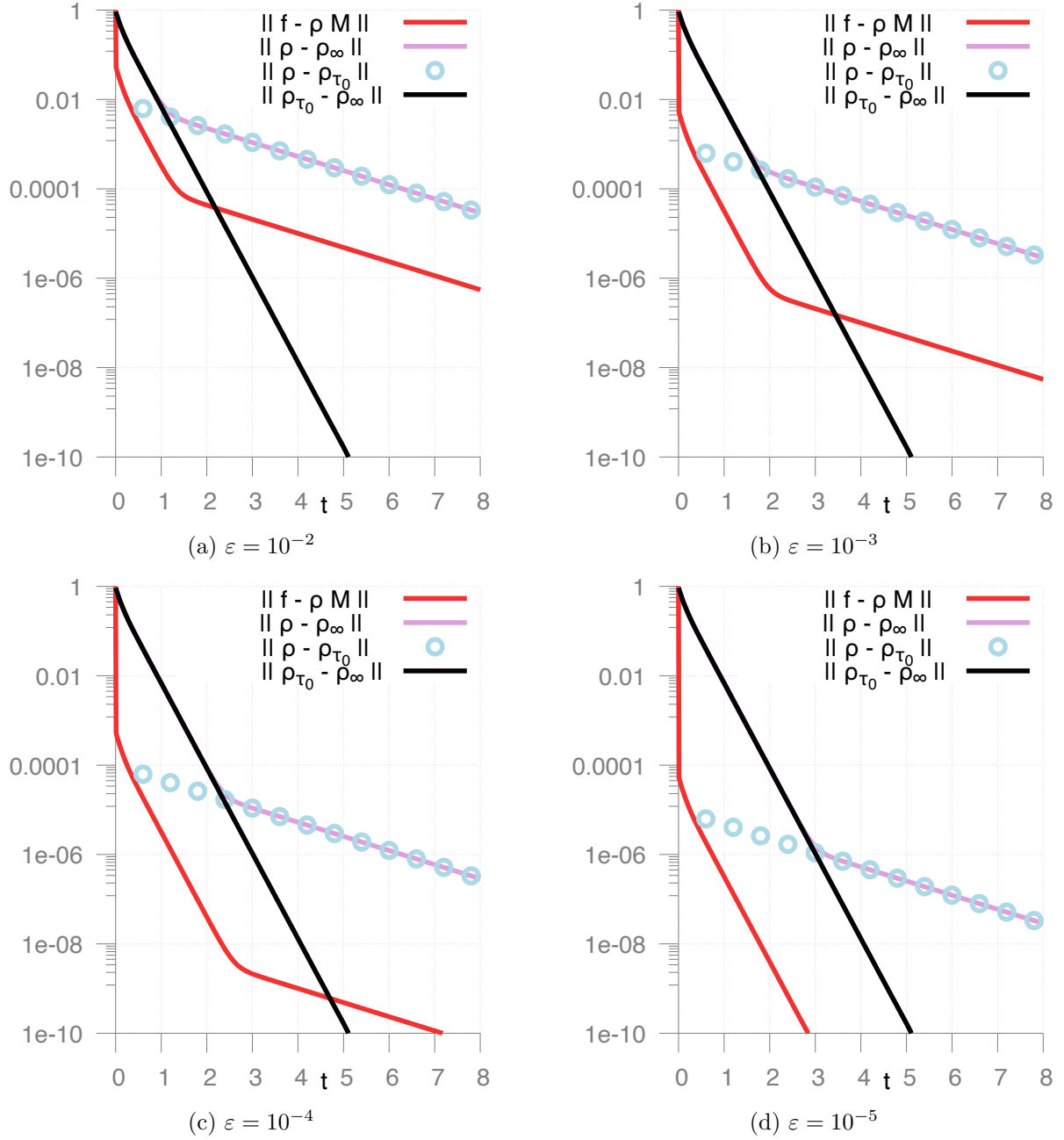
FIGURE 6. Test 2 : shifted Maxwellian. time evolution in log scale of \|f - \rho \mathcal{M}\|_{L^2(f_{\infty}^{-1})} (red), \|\rho - \rho_{\infty}\|_{L^2(\rho_{\infty}^{-1})} (pink), \|\rho - \rho_{\tau_0}\|_{L^2(\rho_{\infty}^{-1})} (blue points) and \|\rho_{\tau_0} - \rho_{\infty}\|_{L^2(\rho_{\infty}^{-1})} (black) for \varepsilon = 10^{-2}, 10^{-3}, 10^{-4} and 10^{-5} .
