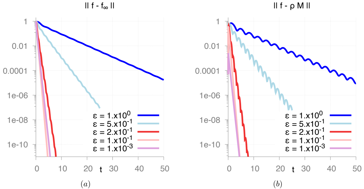
FIGURE 1. Test 1 : centered Maxwellian. time evolution in log scale of (a) \|f - f_\infty\|_{L^2(f_\infty^{-1})} , (b) \|f - \rho \mathcal{M}\|_{L^2(f_\infty^{-1})} .
