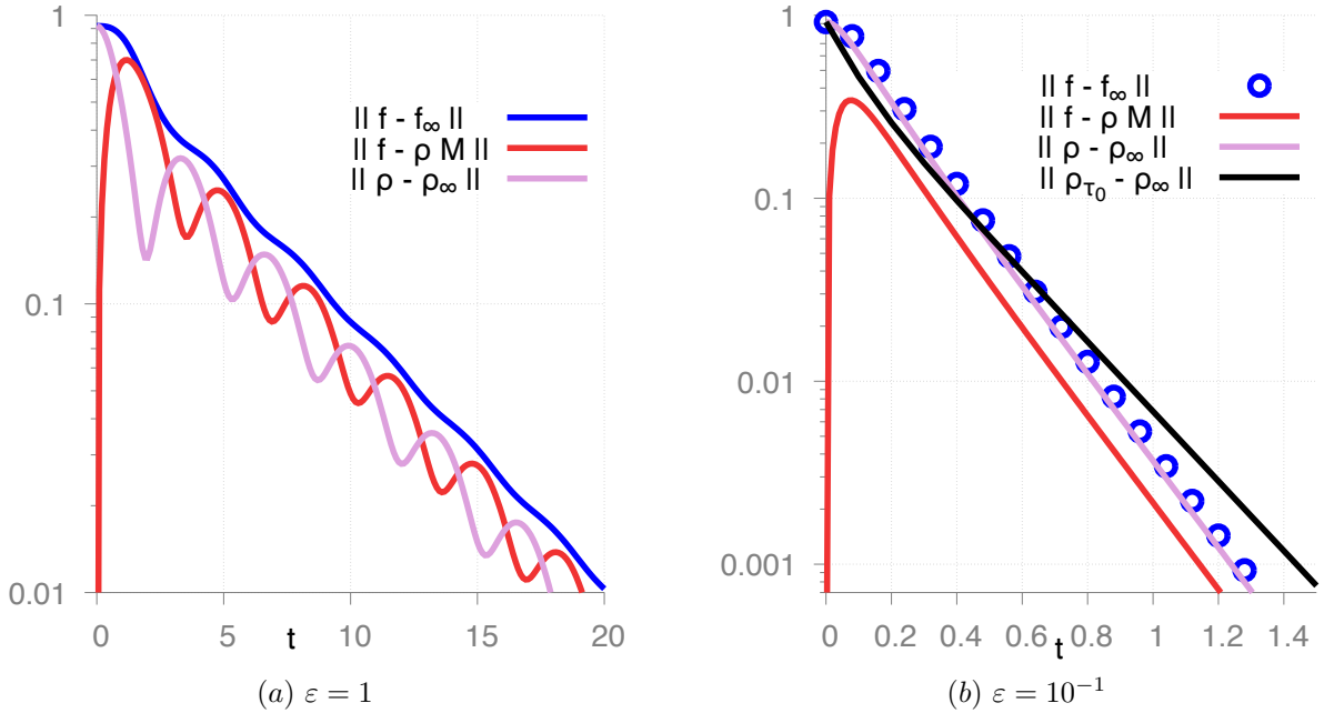
FIGURE 3. Test 1 : centered Maxwellian. time evolution in log scale of \|f - f_\infty\|_{L^2(f_\infty^{-1})} (blue), \|f - \rho \mathcal{M}\|_{L^2(f_\infty^{-1})} (red), \|\rho - \rho_\infty\|_{L^2(\rho_\infty^{-1})} (pink) and \|\rho_{\tau_0} - \rho_\infty\|_{L^2(\rho_\infty^{-1})} (black) for (a) \varepsilon = 1 and (b) \varepsilon = 10^{-1} .
