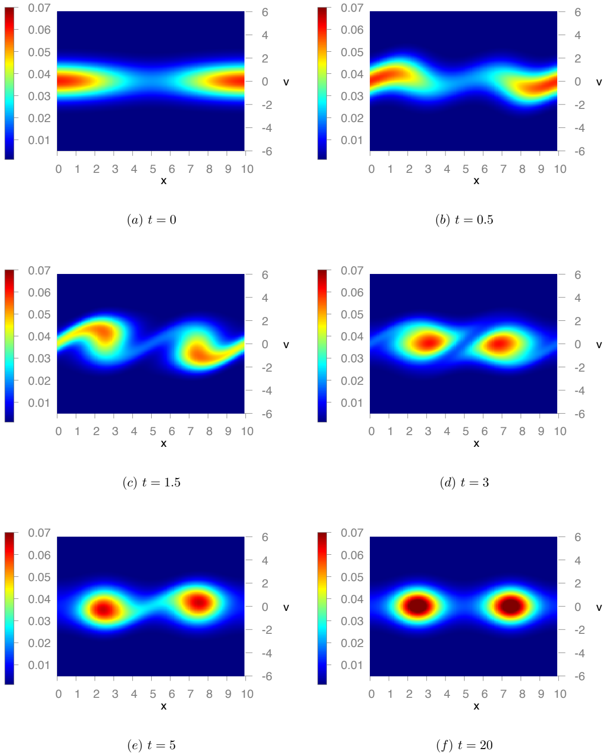
FIGURE 4. Test 1 : centered Maxwellian. snapshots of the distribution function for \varepsilon = 1 at time t = 0, 0.5, 1.5, 3, 5 and 20 .
