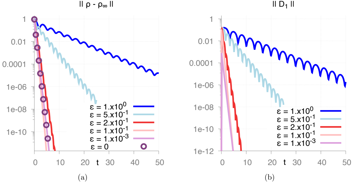
FIGURE 2. Test 1 : centered Maxwellian. time evolution in log scale of (a) \|\rho - \rho_\infty\|_{L^2(\rho_\infty^{-1})} and (b) \|D_1\|_{L^2} .
