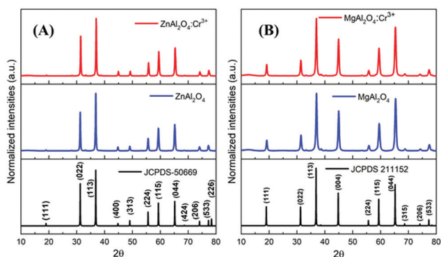
Fig. 2 PXRD patterns of Cr-doped and undoped \text{ZnAl}_2\text{O}_4 (A) and \text{MgAl}_2\text{O}_4 (B). The bottom diagrams are the reference XRD data of the corresponding spinels.
