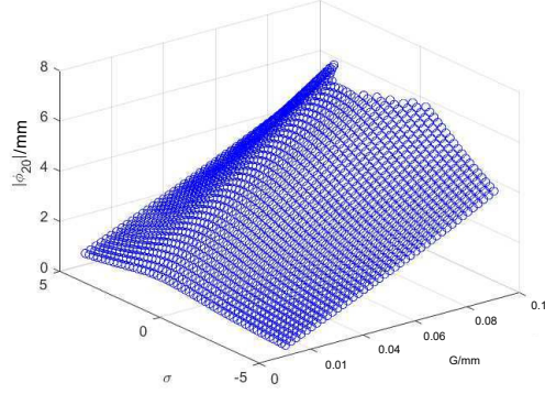
Fig. 3 Amplitude of intra well oscillation in the frequency domain with system parameters: \epsilon = 0.01 , \lambda_1 = 1.67 , \lambda_2 = 0.167 , K = 1742 , \delta = -0.43 . Blue points indicate the stability of the solution.
