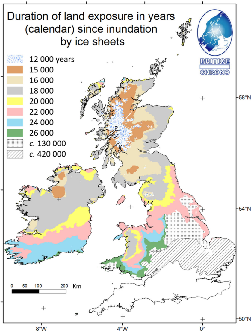
Fig. 19. The duration of time that has elapsed since land has been exposed from beneath ice sheets. Relevant for biological, hydrogeological and archaeological investigations this is based on the BRITICE-CHRONO reconstruction presented earlier, along with younger (Loch Lomond and Nahanagan Stadial) and older (Wolstonian and Anglian) ice cover estimates from Bickerdike et al. (2016), and Gibbard & Clark (2011), respectively.
