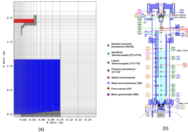
Fig. 2. (a) Representation of the spatial mesh for the numerical experiment. The R -axis is expanded with respect to the Z -axis for better visibility. (b) Representation of the Krotos facility
