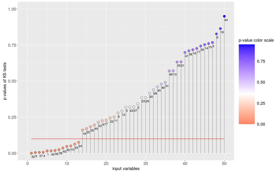
Fig. 3. Ordered p -values of the KS-tests performed for each of the d = 50 inputs.
