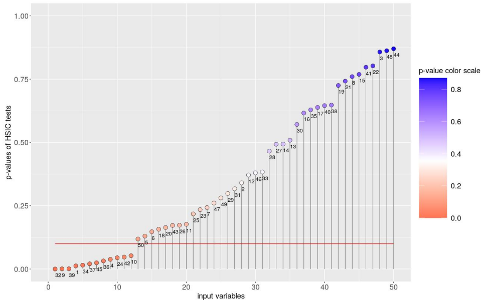
Fig. 4. Ordered p -values associated to HSIC tests of independence performed for each of the d = 50 inputs.
