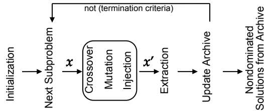
Figure 1: The MOEA/D learning framework.
