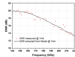
Fig. 7: Simulated and measured ENR curve of the diode of size 3.44\mu\text{m}^2 biased at 7mA.
