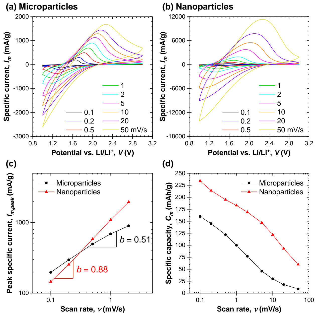
Figure 3: Cyclic voltammogram of Swagelok cells with working electrodes made of \text{Ti}_2\text{Nb}_2\text{O}_9 (a) microparticles or (b) nanoparticles cycled between 1.0 and 3.0 V vs. \text{Li}/\text{Li}^+ at scan rates \nu ranging between 0.1 and 50 mV/s, along with (c) peak specific current I_{m,peak}(\nu) , and (d) specific capacity C_m(\nu) as functions of scan rate \nu .
