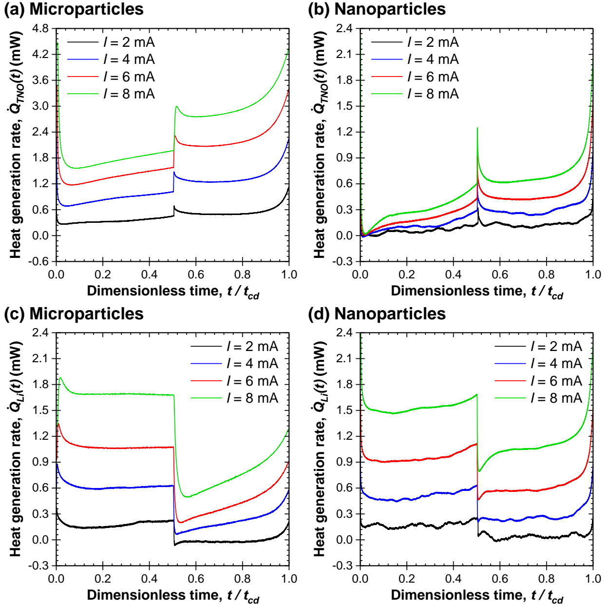
Figure 7: Instantaneous heat generation rates (a, b) \dot{Q}_{TNO}(t) measured at the working electrodes made of Ti_2Nb_2O_9 microparticles or nanoparticles and (c, d) \dot{Q}_{Li}(t) measured at the corresponding lithium metal counter electrodes as functions of dimensionless time t/t_{cd} averaged over the last three consecutive cycles for current I ranging from 2 to 8 mA.
