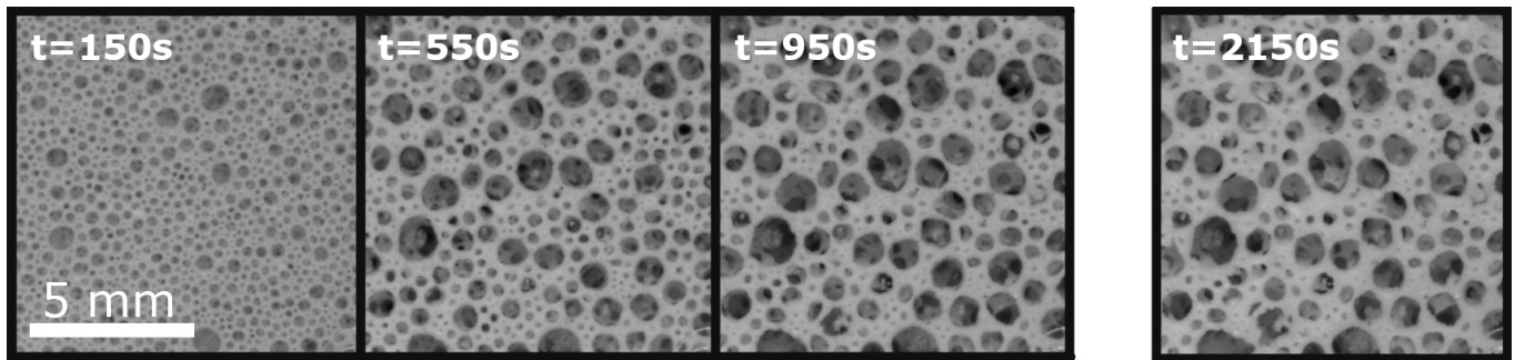
Figure 3. Evolution of the foam top surface with time t . Experimental conditions: t_m = 60 s, \omega_m = 17 Hz, surfactant concentration 3 g/L, citric acid concentration c_{CA} = 0.5 g/L.
