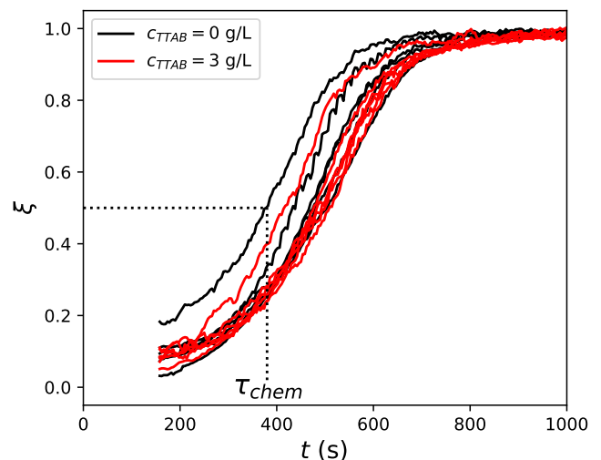
Figure 5. Extent of the reaction \xi as a function of time t with TTAB surfactant (light red) and without surfactant (black). Each experiment was repeated 6 times. Final W/P = 1. Experimental conditions: t_m = 60 s, \omega_m = 7 Hz, no citric acid.
