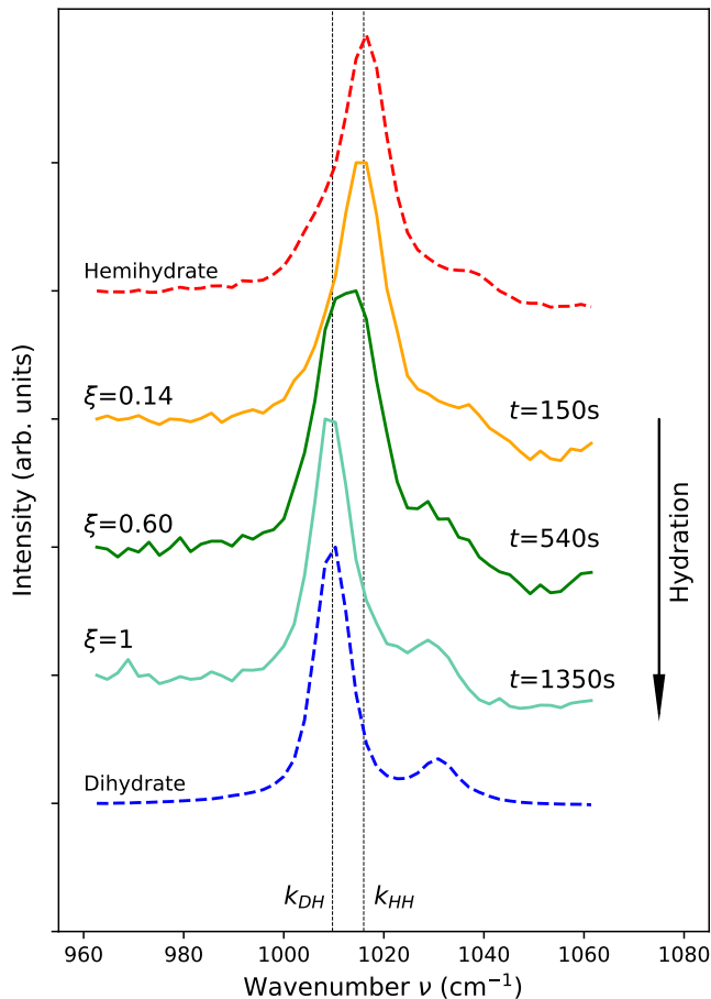
Figure 4. Raman spectra showing the transition of peak \nu_1(\text{SO}_4) during the hydration reaction in a foamed sample ( t_m = 60 s, \omega_m = 17 Hz, TTAB 3 g/L, no citric acid): intensity (offset for clarity) as a function of the Raman shift wavenumber \nu . Plain lines correspond to the Raman peak of the foamed plaster at t = 150 , 540 and 1350 s, corresponding to extent of reaction \xi = 0.14 , 0.60 and 1 respectively. Dashed lines correspond to hemihydrate (plaster) and dihydrate (gypsum) Raman band as measured separately on powders. k_{\text{HH}} and k_{\text{DH}} are the corresponding peak positions.
