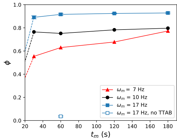
Figure 2. Air volume fraction \phi incorporated in the foamed plaster suspension, as a function of the mixing time t_m for different mixing rates \omega_m . Dashed lines show the extrapolation to \phi = 0 when the suspension is not mixed ( t_m = 0 s). TTAB surfactant solution is used at concentration 3 g/L, except for the hollow square (no surfactant). The errorbars for \omega_m = 17 Hz illustrate the reproducibility of the measurement.
