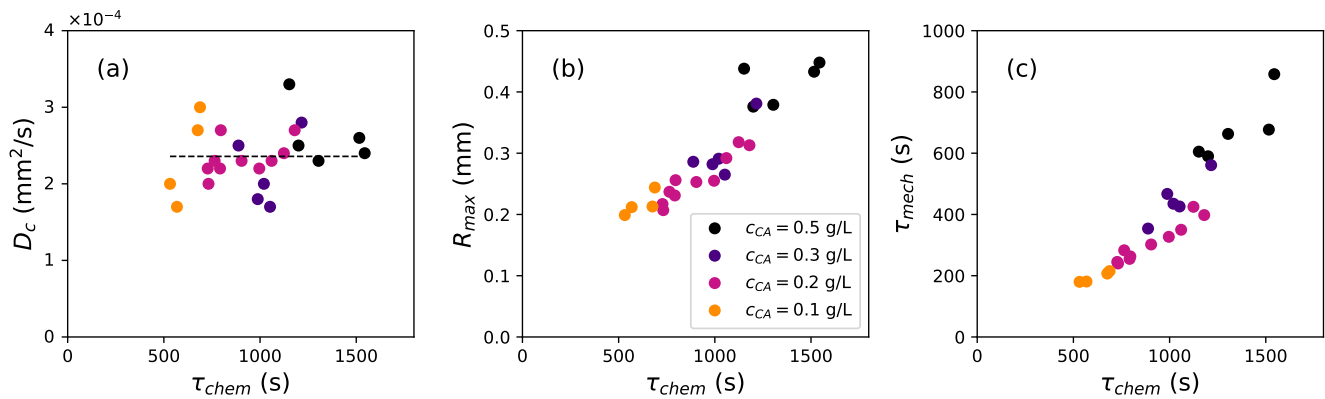
Figure 10. (a) Effective diffusion coefficient D_c for coarsening dynamics, (b) maximum Sauter radius R_{\max} and (c) mechanical time for coarsening arrest \tau_{\text{mech}} , as a function of the hydration time \tau_{\text{chem}} for various citric acid concentrations c_{\text{CA}} (colors). The horizontal line in (a) shows the average value D_c = (2.4 \pm 0.4) \cdot 10^{-4} \text{ mm}^2/\text{s} . Experimental conditions: t_m = 60 \text{ s} , \omega_m = 17 \text{ Hz} , foamed samples (surfactant TTAB at 3 g/L).
