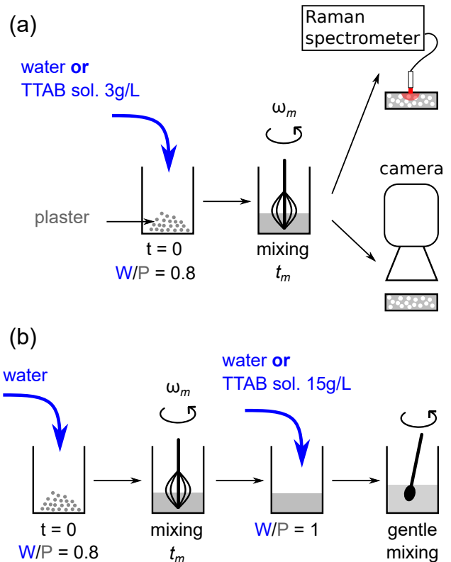
Figure 1. (a) Preparation protocol used in most of our experiments. (b) Special protocol to study the influence of the surfactant (see text for details).
