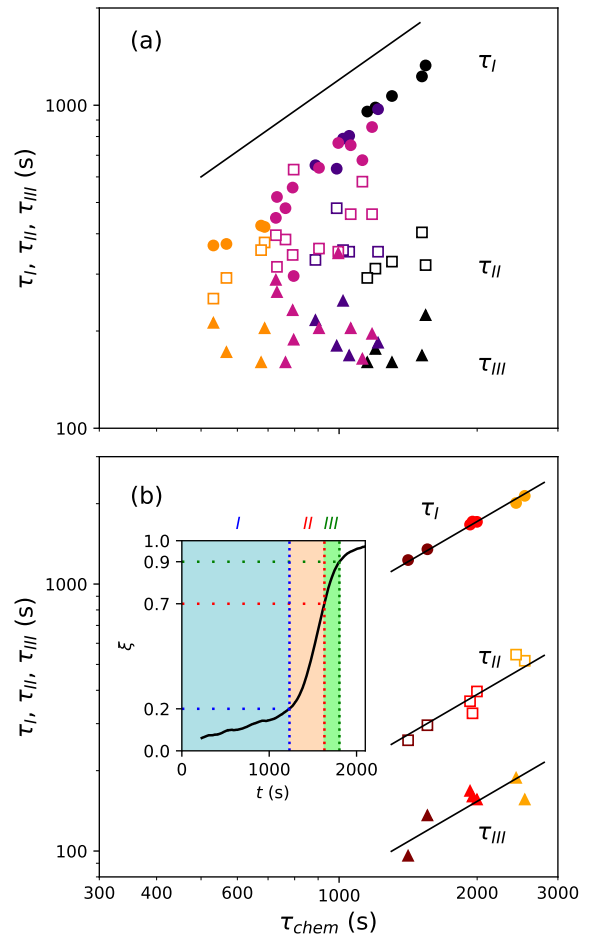
Figure 9. Characteristic timescales of the three phases of hydration \tau_I (induction), \tau_{\text{II}} (growth-limited) and \tau_{\text{III}} (dissolution-limited), as a function of the average duration \tau_{\text{chem}} . (a) Influence of the citric acid concentration, increasing from left to right (same colors as in figure 8). The line corresponds to a linear behaviour \tau \sim \tau_{\text{chem}} . (b) Influence of the mixing duration t_m , decreasing from left to right (same colors as in figure 6), c_{\text{CA}} = 0.5 \text{ g/L} , \omega_m = 7 \text{ Hz} . The lines show the linear fits of the data. Inset: typical hydration curve \xi(t) highlighting the three phases of the reaction.
