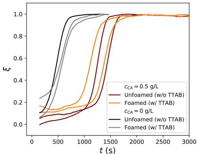
Figure 7. Extent of the reaction \xi as a function of time t for c_{\text{CA}} = 0 and 0.5 g/L. Samples are either foamed (with surfactant TTAB at concentration 3 g/L) or unfoamed (without surfactant). Experimental conditions: t_m = 60 s, \omega_m = 17 Hz.
