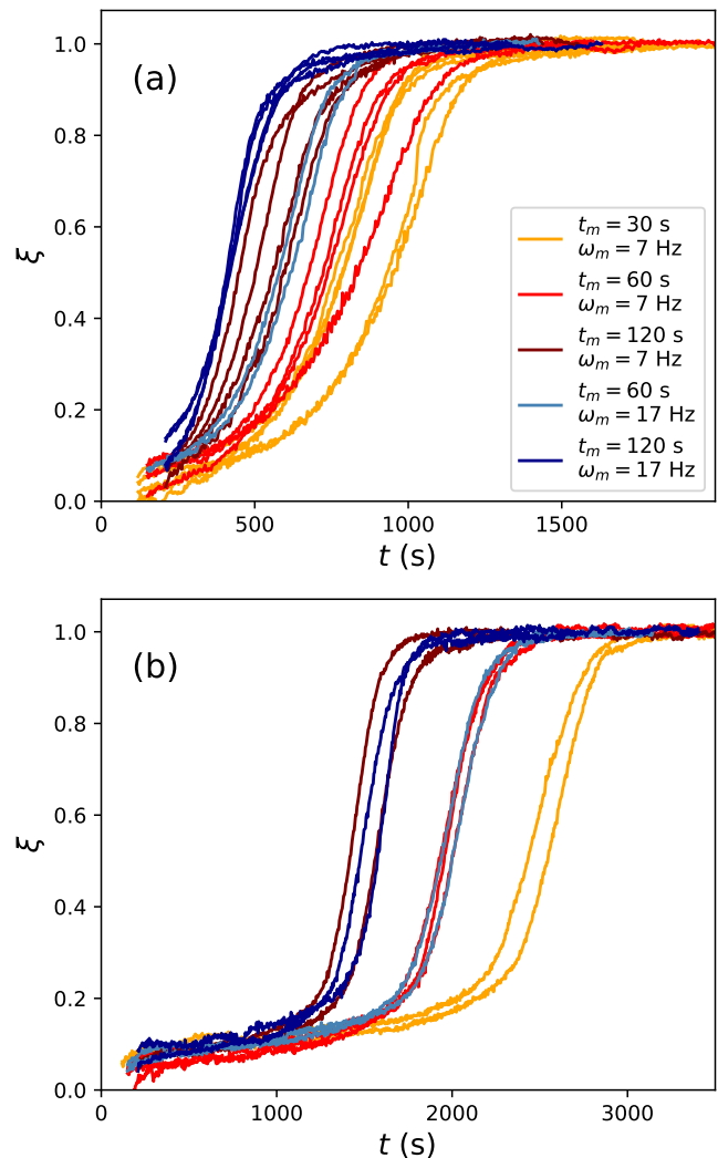
Figure 6. Extent of the reaction \xi as a function of time t for different mixing times t_m , mixing rates \omega_m and citric acid concentrations (a) c_{\text{CA}} = 0 and (b) c_{\text{CA}} = 0.5 g/L. Several experiments are done in the same conditions to illustrate the reproducibility of the measurements. No surfactant is used so the samples are unfoamed. The measurements were obtained at a fixed location in the sample (no turntable).
