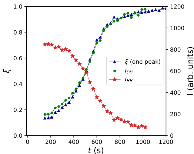
Figure 12. Evolution of hemihydrate I_{HH} and dihydrate I_{DH} intensities (right axis, from two peak analysis), together with the extent of reaction \xi (left axis, one peak analysis). Experimental conditions: foamed and turned sample without retardant, t_m = 60 s, \omega_m = 17 Hz. The time interval between two measurements is 30 s.
