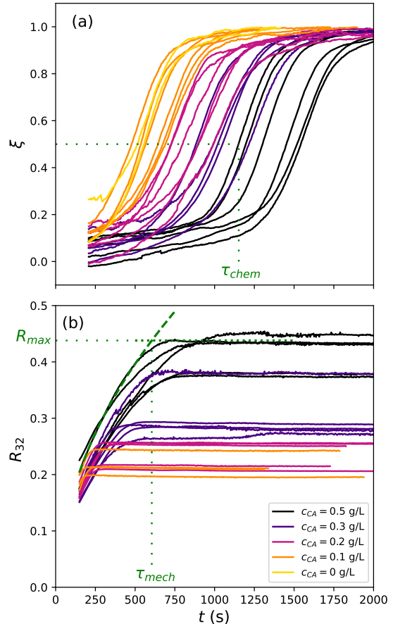
Figure 8. (a) Extent of the reaction \xi as a function of time t for different citric acid concentrations c_{\text{CA}} . The dashed lines show the definition of \tau_{\text{chem}} for one specific experiment. (b) Sauter radius R_{32} as a function of time for different citric acid concentrations c_{\text{CA}} . For the same specific experiment as in (a), the dashed line corresponds to a fit by equation 3 for coarsening dynamics, with D_c = 3.3 \cdot 10^{-4} mm 2 /s (see section IV B). The dotted line shows the maximum radius R_{\text{max}} obtained at the end of the experiment. \tau_{\text{mech}} is defined as the intercept between the two curves and characterizes the arrest of coarsening of each experiment. Experimental conditions: t_m = 60 s, \omega_m = 17 Hz, TTAB concentration 3 g/L.
