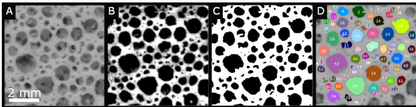
Figure 11. Image processing method. A: raw image, B: subtracted image (grayscale adjusted for clarity), C: binary image, D: detected bubbles (numbered). Experimental conditions: t = 1750 s, t_m = 60 s, \omega_m = 17 Hz, TTAB 3 g/L, c_{CA} = 0.5 g/L.
