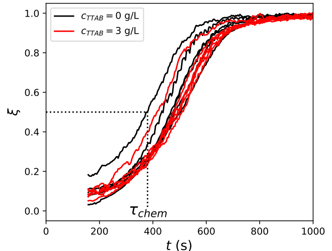
Figure 5. Extent of the reaction \xi as a function of time t with TTAB surfactant (light red) and without surfactant (black). Each experiment was repeated 6 times. Final W/P = 1. Experimental conditions: t_m = 60 s, \omega_m = 7 Hz, no citric acid.
