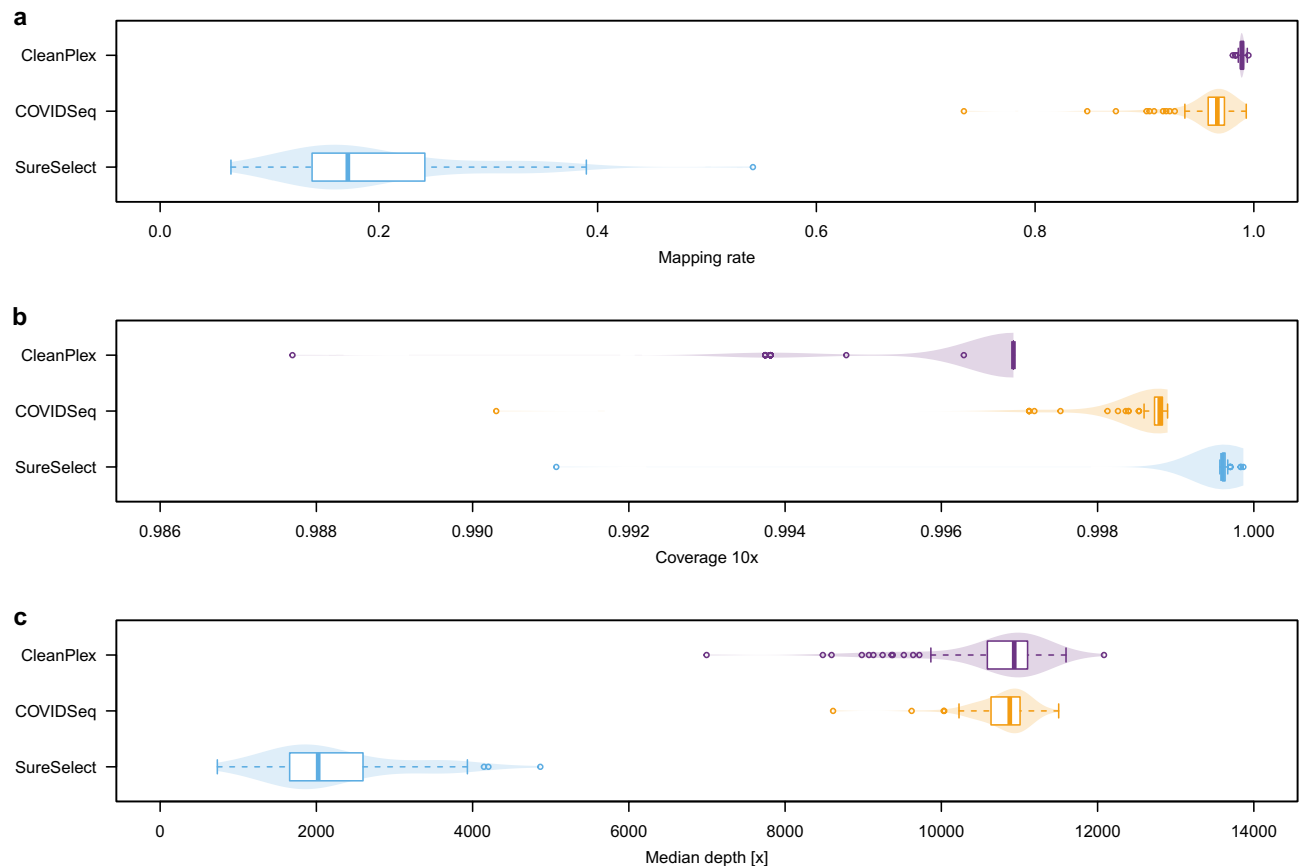
Figure 1. Comparison of target enrichment kits performance. (a) SARS-CoV-2-specific mapping rate. (b) Breadth of coverage of the SARS-CoV-2 genome, where the depth of coverage is at least 10×. (c) Median depth of coverage.
