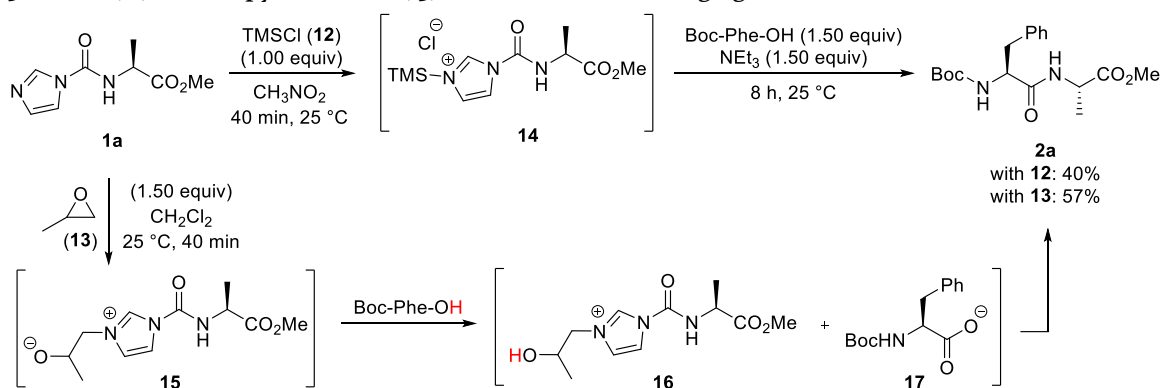
Scheme 5. TMSCl (12) and Propylene Oxide (13) as Imidazole Activating Agents
