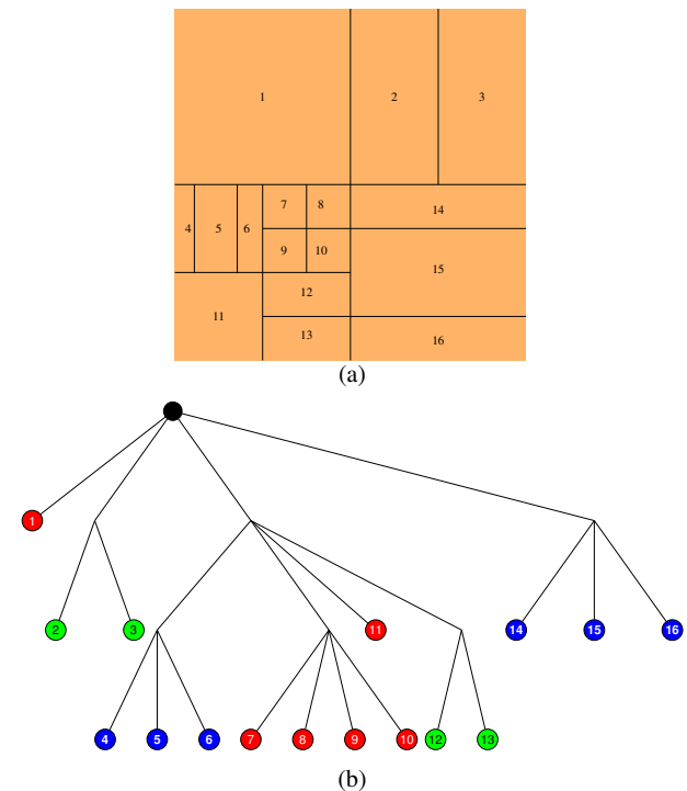
Figure 1: Example of QTBT partition of the CTU. (a) QTBT partition of the CTU in blocks. (b) Corresponding tree representation of the CTU : Quad-tree (in red), binary-tree (in green) and ternary-tree (in blue) splits.
