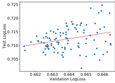
(c) Slope: 1.00 - R^2 : 0.08 - Test year 2018
