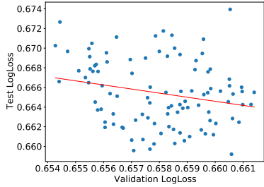
(a) Slope: -0.42 - R^2 : 0.05 - Test year 2016
