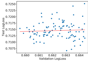
(e) Slope: 0.14 - R^2 : 0.00 - Test year 2020
