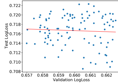
(b) Slope: -0.12 - R^2 : 0.00 - Test year 2017
