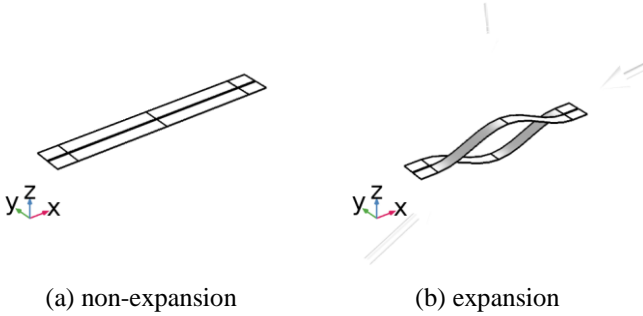
Fig. 2. 3D deformation diagrams of REBCO ring tape
