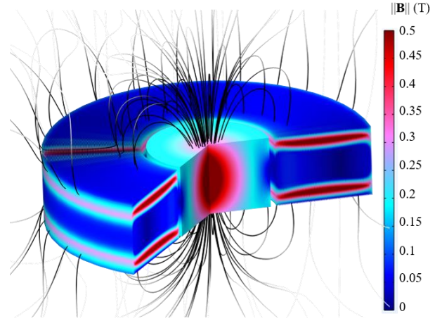
Fig. 4. 3D view of the PTF at the end of the energization process at 77 \text{ K} , where the norm of the magnetic flux density is presented both in the (RE)BCO bulk and the HTSc tape for I_{\text{max}}/I_c = 0.9 and 80 turns.
