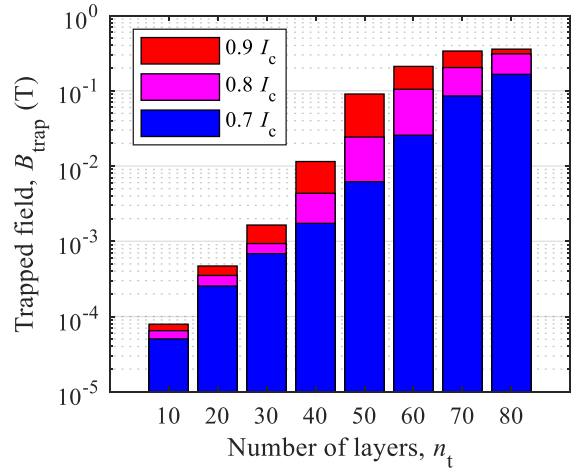
Fig. 5. Trapped field at the center of the top surface of the (RE)BCO bulk at 77 \text{ K} as a function of the number of layers of the HTSc tape and for different values of I_{\text{max}} .
