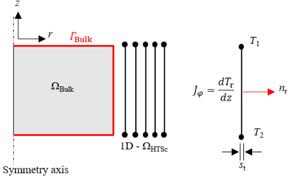
Fig. 3. The thickness of the HTSc tape is reduced to a surface current density (1D element). The current is imposed by boundary conditions at the T_1 and T_2 edges of the tape. \Gamma_{\text{Bulk}} is the boundary between the two regions (Bulk and Air).
