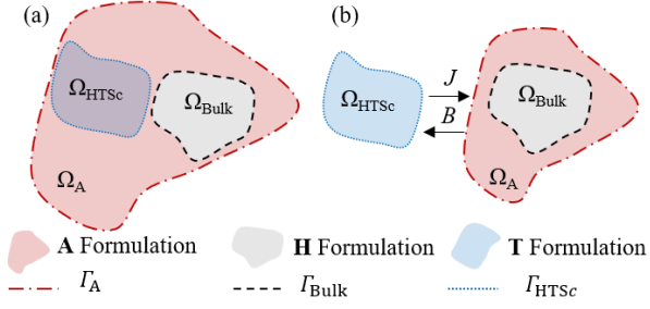
Fig. 2. (a) Representation of the different fields of study: \mathbf{H} is calculated only in the bulk (gray), \mathbf{T} is calculated only in the superconducting domain (blue), while \mathbf{A} is calculated in air (light red). (b) Coupling between \mathbf{T} and \mathbf{A} - \mathbf{H} formulations in the simulation. \mathbf{J} and \mathbf{B} are the two coupling variables.
