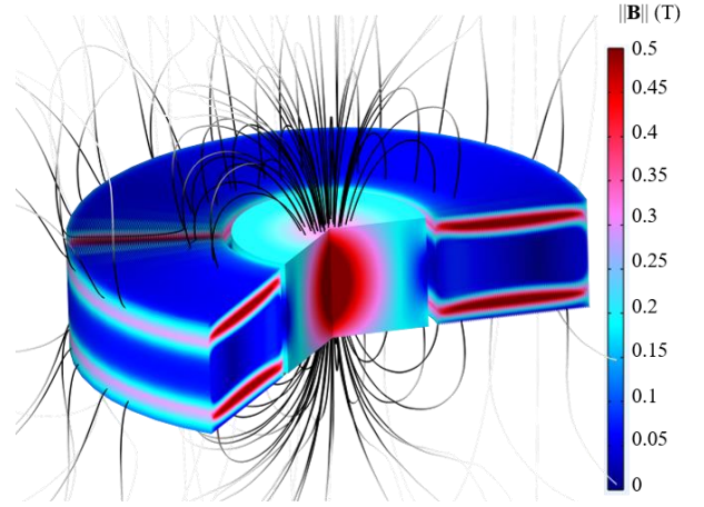
Fig. 4. 3D view of the PTF at the end of the energization process at 77 \text{ K} , where the norm of the magnetic flux density is presented both in the (RE)BCO bulk and the HTSc tape for I_{\text{max}}/I_c = 0.9 and 80 turns.
