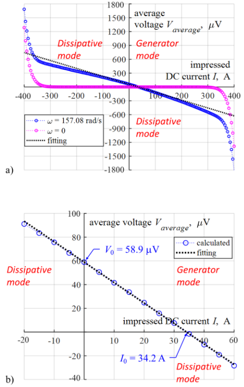
Fig. 1. A) Average voltage of the flux pump rotating at 157.08 rad/sec (25 Hz) compared with the voltage developing at the tape's terminal in case of no rotation. The dotted line represents the linear V-I trend. b) Magnification the V-I points in the first quadrant.
