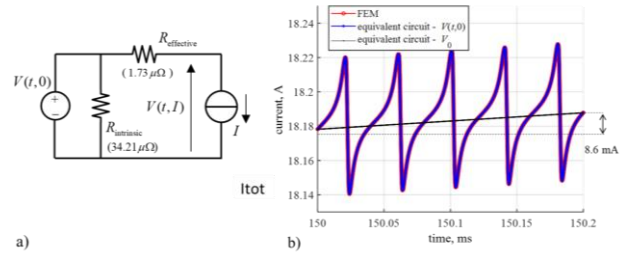
Fig. 2. a) complete time-domain empirical equivalent circuit of the flux pump taking internal dissipation into account, b) Detail of the current during 5 cycles.
