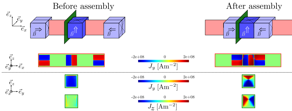
Fig. 1. Comparison of the y - and z -components of the current density distribution before and after the assembly of the superconducting Halbach array computed with the finite-element model. The results are presented in two different cut planes represented in red and green respectively.
