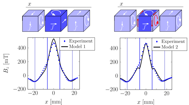
Fig. 2. Evolution of the z -component of the magnetic flux density generated 1 mm away from the surface of a Halbach array made up of three cuboid bulk superconductors along the line x . The analytical model considers a simple vector summation of the flux densities generated by each superconductors in the array, square current loops strictly perpendicular to the magnetization direction and a constant and field-independent critical current density. Model 1 assumes no alteration of initial current density distribution. Model 2 includes the modifications predicted by the finite-element simulation.
