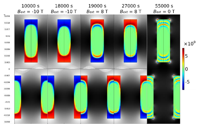
Fig. 1 – Simulated magnetization currents in a single period of a superconducting undulator at different time steps of the simulation.
