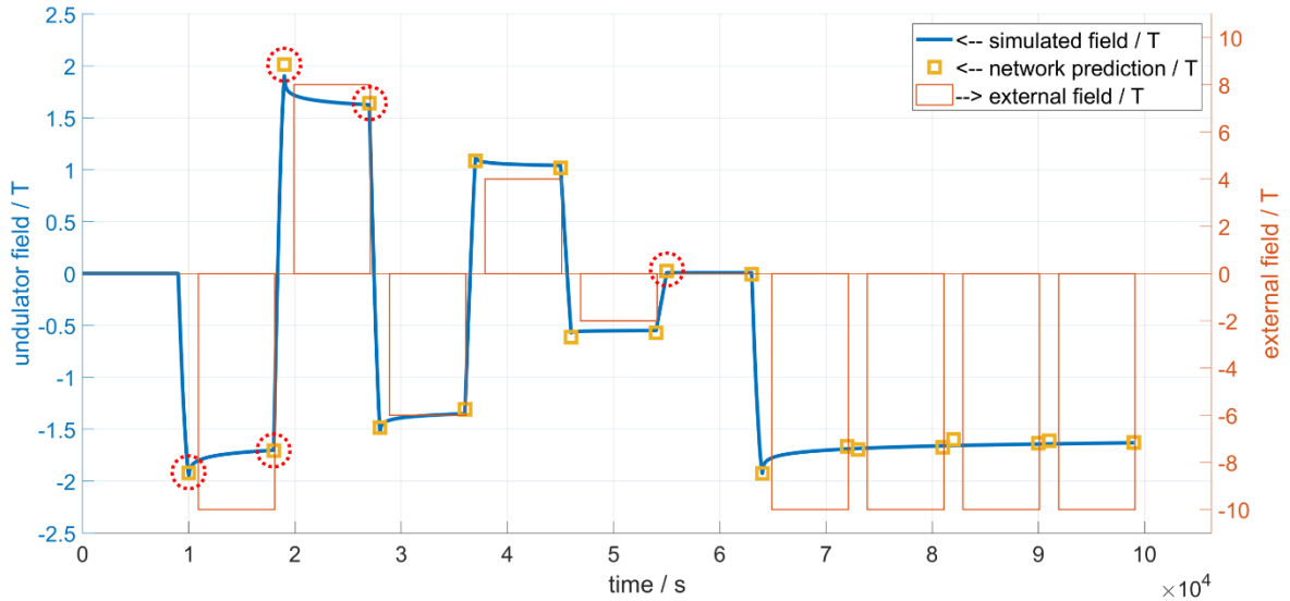
Fig 2. Evaluation of the trained neural network predicting the undulator field depending on the applied external field and the external field history. The dotted circles indicate the time steps depicted in Fig.1
