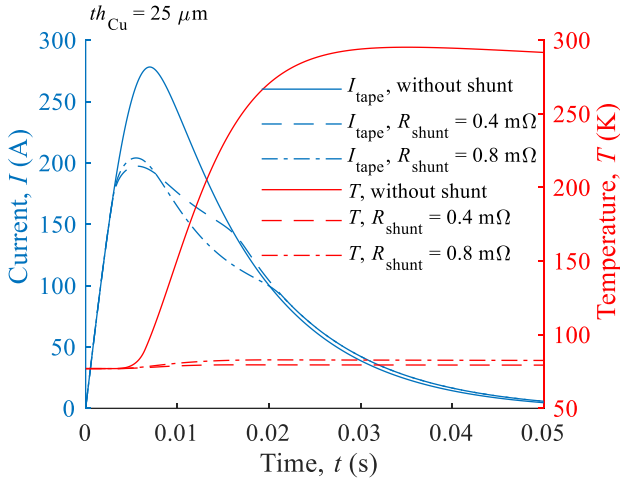
Figure 4. Tape current and temperature as a function of time, with a copper layer thickness of 25 \mu\text{m} , without shunt in parallel to the HTS tape and for two different values of R_{\text{shunt}} .
