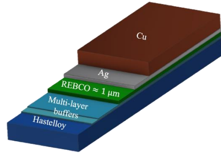
Figure 2. View of the different layers of a typical 2G HTS tape.
