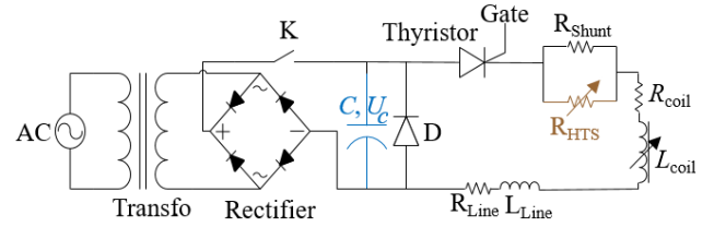
Figure 1. Circuit diagram of the pulse current supply for a HTS tape.
