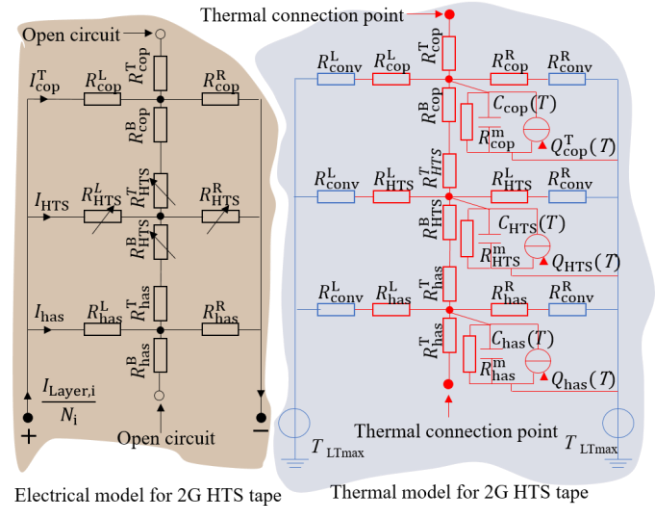
Figure 3. Diagram of the electro-thermal model of a 2G HTS tape.
