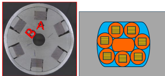
Fig. 1 Cross-section of HTS conductor concepts proposed by ENEA and SPC.
