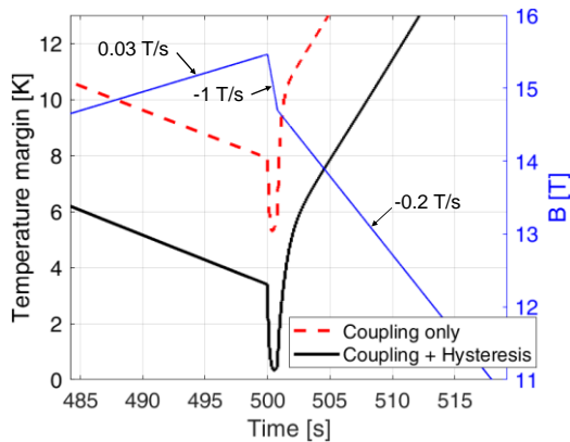
Fig. 3 Evolution of the temperature margin when coupling losses only or when coupling and hysteresis losses are considered. The magnetic field and its ramp rates are also reported
