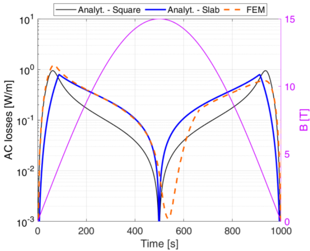
Fig. 2 Evolution of the losses computed with analytical and FEM models. The evolution of the magnetic field is reported in magenta.
