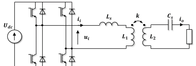
Fig. 1. Lumped circuit model of HTS wireless power transmission system.
