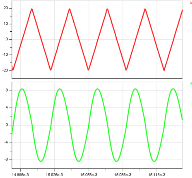
Fig. 2. Current waveforms obtained from lumped circuit model. Current of transmitter (red), and receiver (green).
