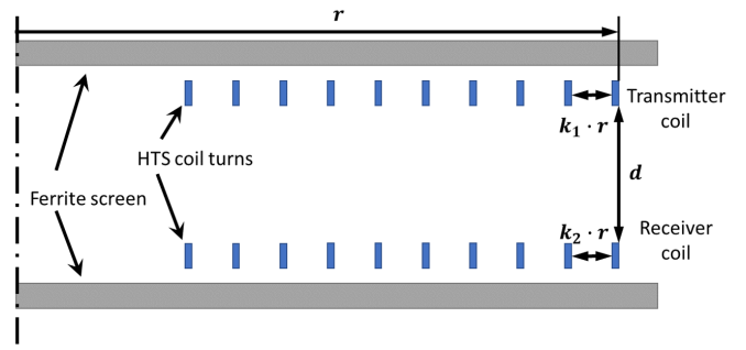
Fig. 3. Finite-element model geometry.
