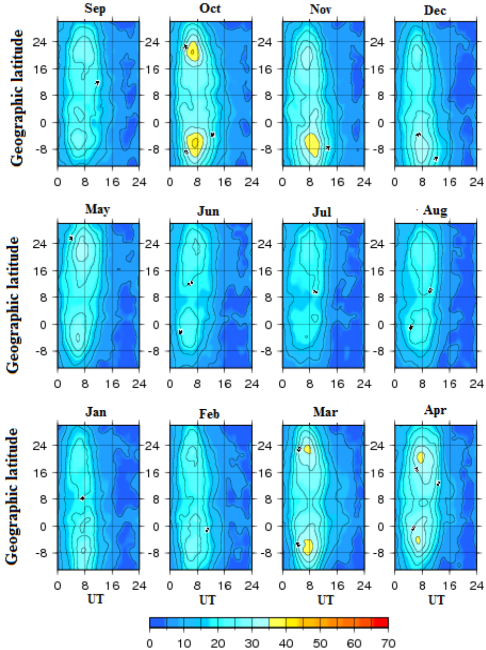
Figure 2. The temporal-litudinal monthly average TEC maps in 2009. Contour interval of 5 TECU
