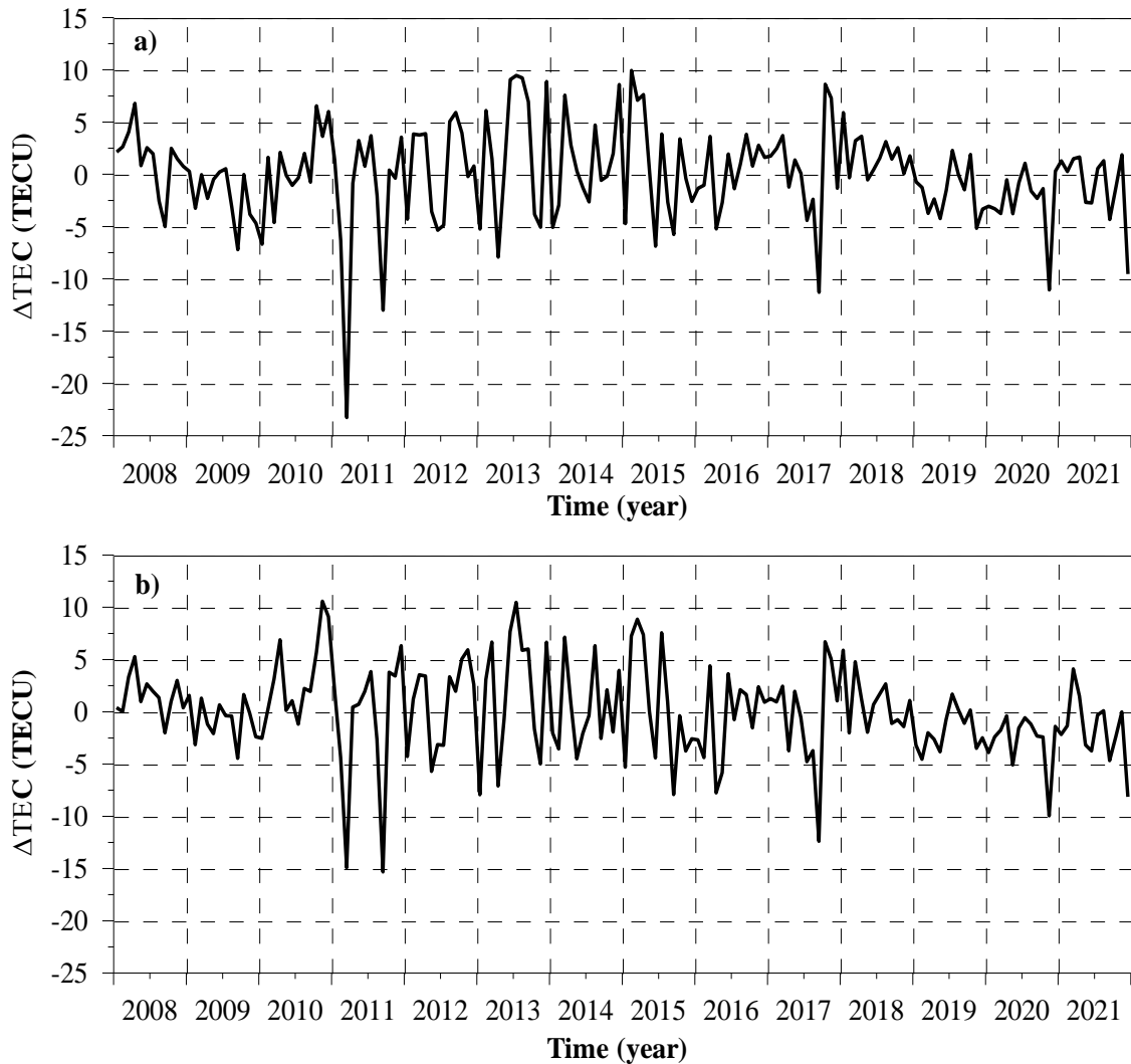
Figure 5. The variation of \Delta\text{TEC} residuals after subtracting the amplitudes fitted with F10.7 from monthly mean EIA crests amplitudes for the period 2008-2021 a) for the northern crest, b) for the southern crest
