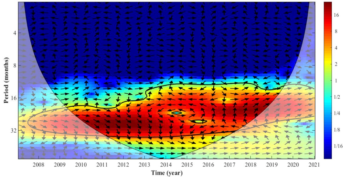
Figure 9. The same as Fig. 8 for the southern crest
