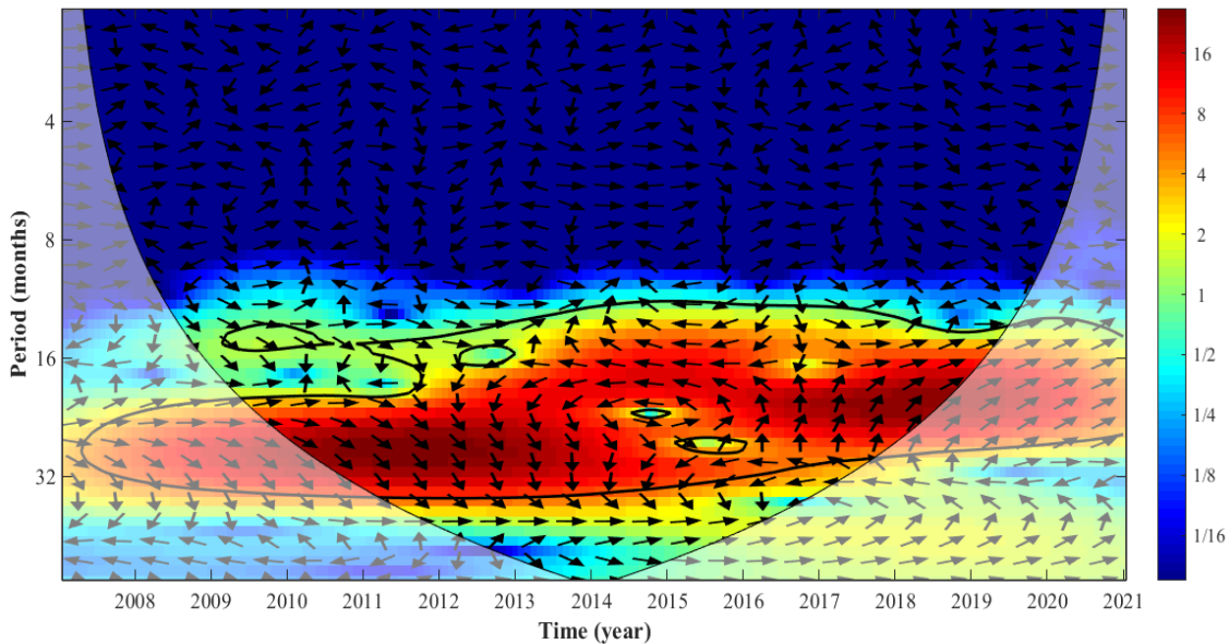
Figure 8. Cross-wavelet transform of the ionosphere QBO of the northern crest and the SQBO. The 95% confidence is shown as a thick contour; the cone of influence (COI), where edge effects might
