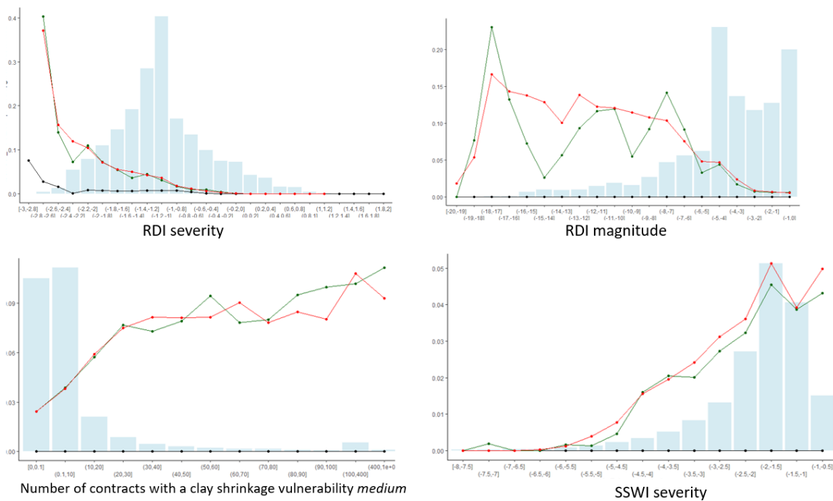
(a) One way-analysis for GLM CatNat.
