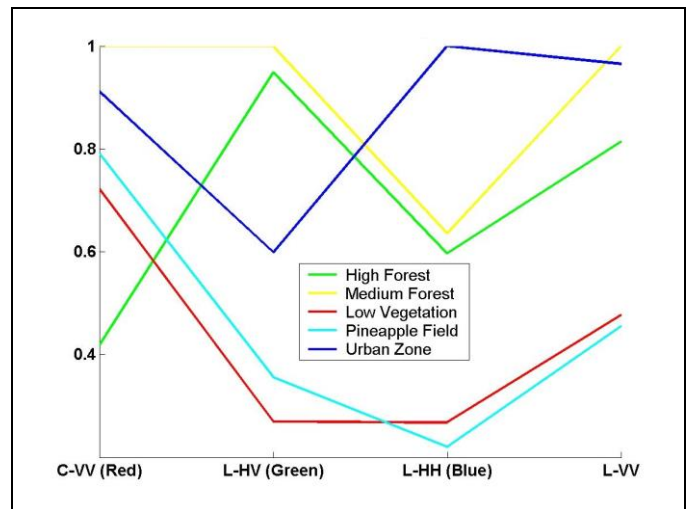
Figure 4. AirSAR Classes Mean Signature (Normalized)
