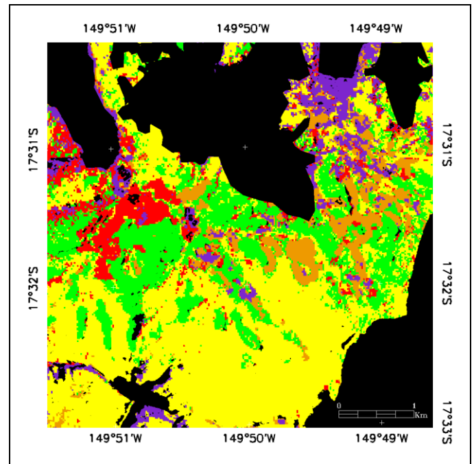
Figure 6. Opunohu Valley MASTER Classification Map
