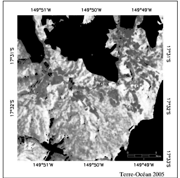
Figure 6. MASTER NDVI Vegetation Index Map
