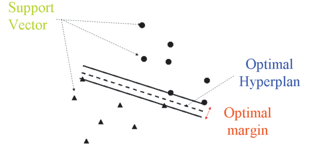
Fig. 1. SVM Classifier-Linear case
