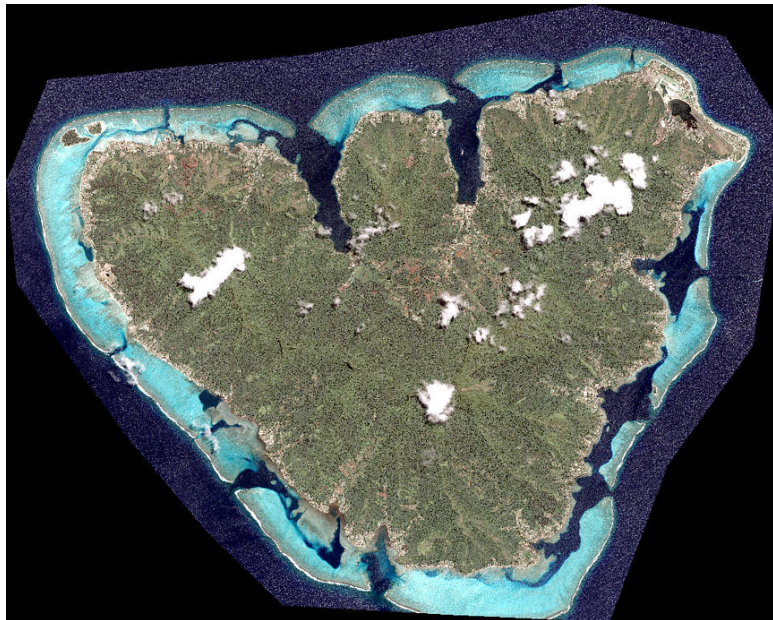
Figure 1. 2002 Moorea Quickbird RGB image.
