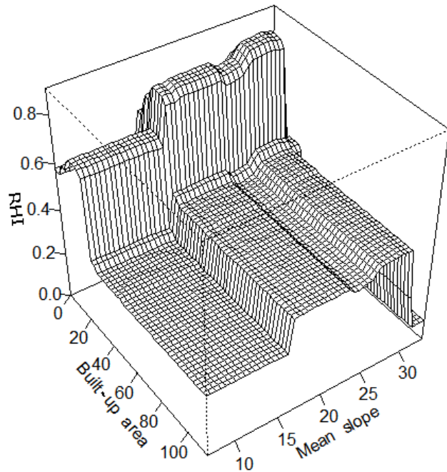
Figure 2: Joint partial dependence plots between the RHI score and explanatory variables provided with the largest RI.
