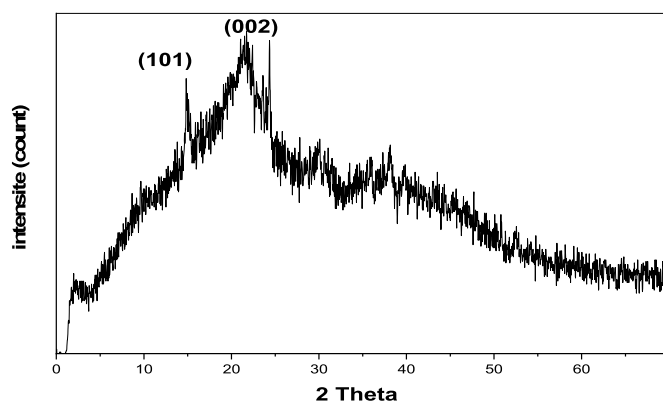
Fig. 2. XRD pattern of Raw Aloe vera powder.
