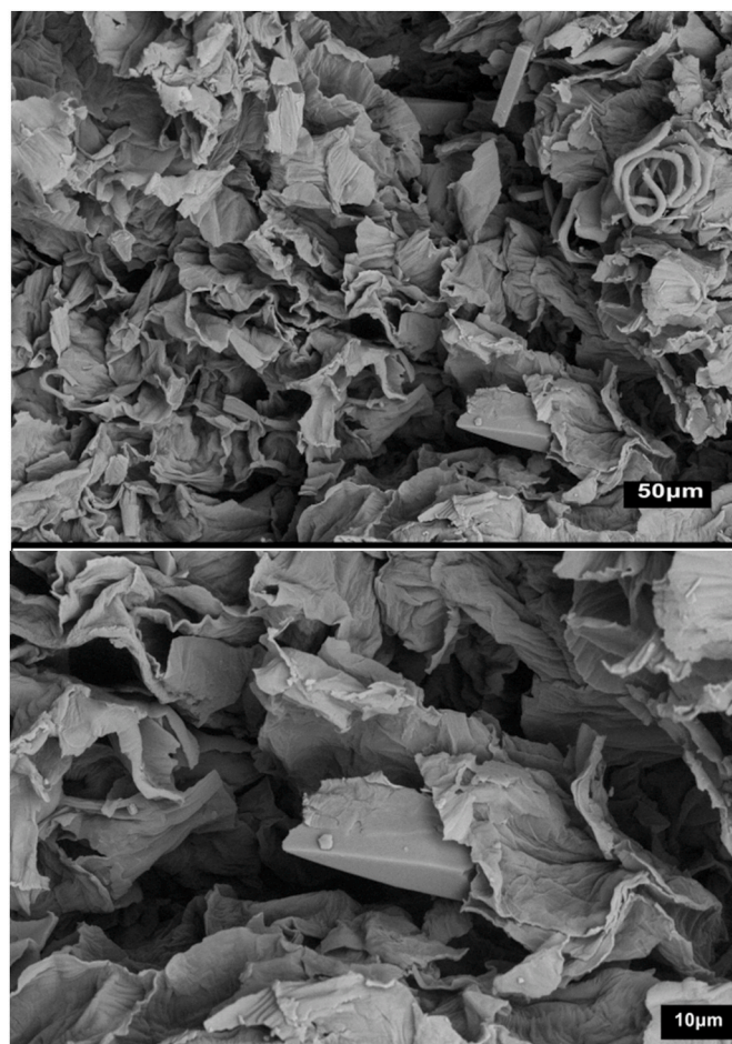
Fig. 3. SEM image of AV (a) at 50 \mu\text{m} and (b) 10 \mu\text{m} .
