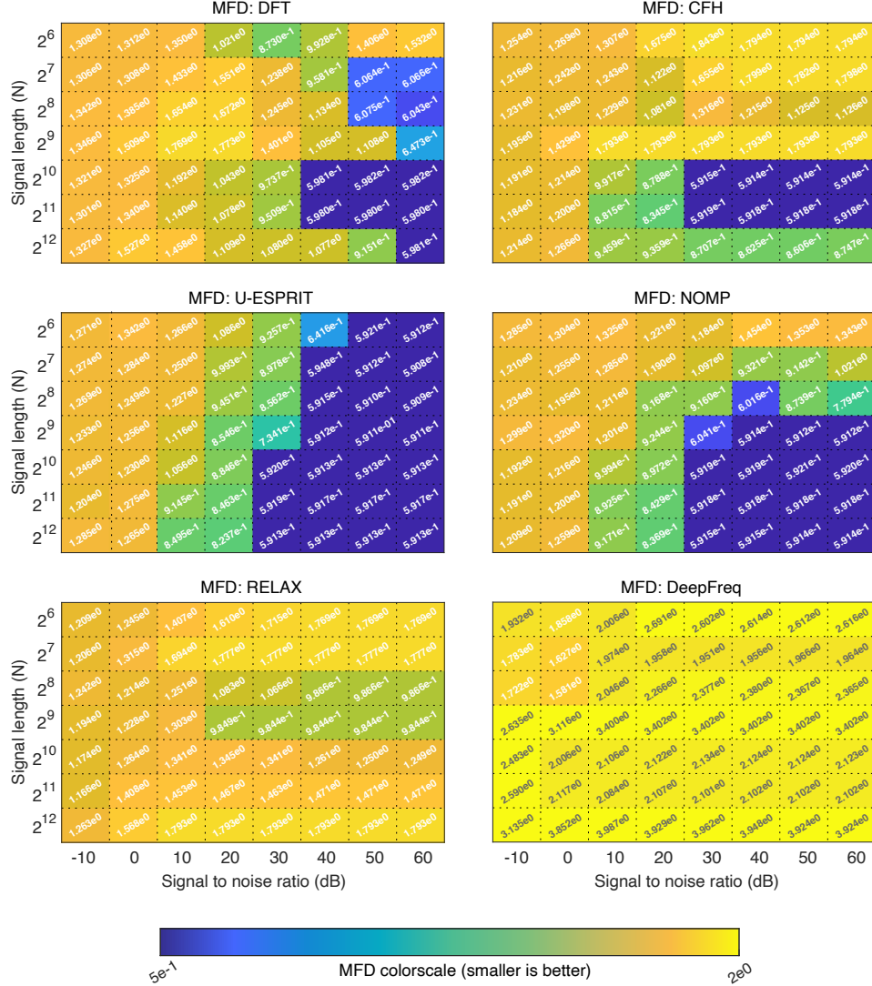
Figure 10: Simulation results as heatmaps of the MFD metric for each LSE, whose colorscales are plotted logarithmically.
