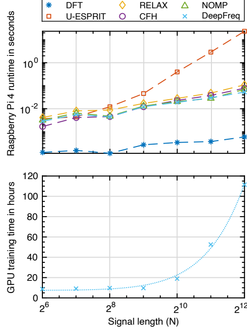
Figure 15: Averaged runtimes of LSEs on a Raspberry Pi 4 (top) and offline Tesla P100 GPU training time required for frequency representation module of DeepFreq (bottom) with respect to signal length N . The legend shown above applies to all plots.
