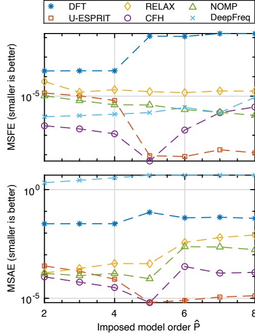
Figure 14: Simulation results for varying imposed model orders \hat{P} . The signal length N = 2^7 , SNR = 40 dB, amplitude magnitude ratio \alpha = 1.5 , and model order P = 5 are pre-determined. The legend shown above applies to all plots.
