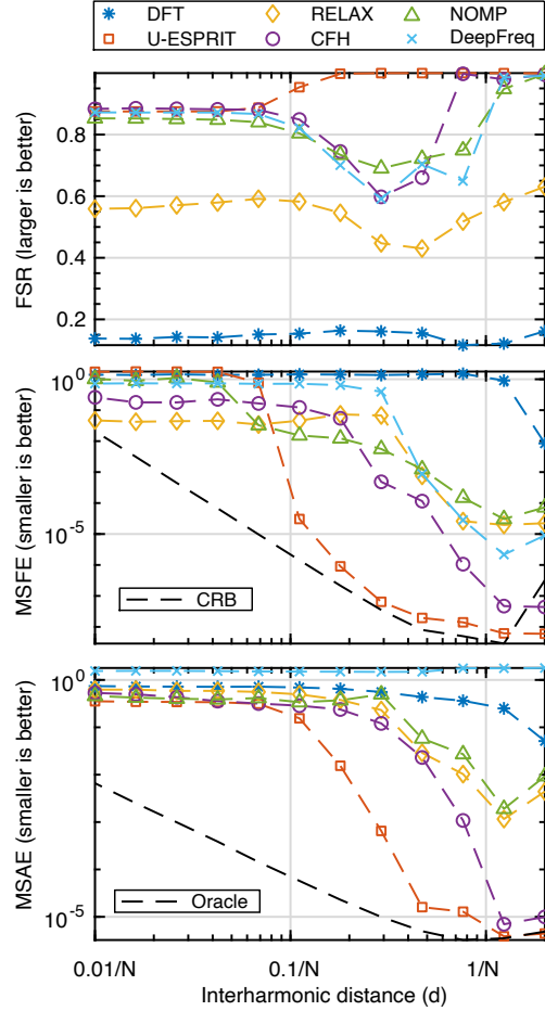
Figure 13: Simulation results for varying interharmonic distance parameter d . The signal length N = 2^7 , SNR = 40 dB, amplitude magnitude ratio \alpha = 1.5 , and model order P = 3 + 1 are pre-determined. The legend shown above applies to all plots, with sub-legends within the plots applying only to sub-plots.
