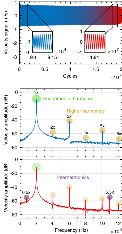
Figure 2: (Top) Velocity signal from a typical ultrasonic fatigue test with segmented signal windows near the beginning and end of the fatigue test. Frequency spectra corresponding to an undamaged (center) and damaged (bottom) fatigue specimen are obtained through a DFT. Harmonics correspond to integer multiples of the fundamental harmonic while interharmonics correspond to non-integer multiples of the fundamental harmonic.
