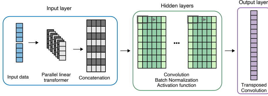
Figure 5: Architecture of the DeepFreq frequency representation module.
