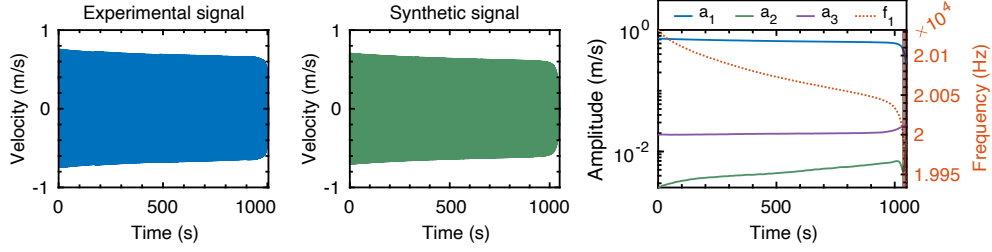
Figure 6: Copper specimen ultrasonic fatigue test excited at 20 kHz with vibration signal sampled at 200 kHz (left). A synthetic signal (center) is created from the first 3 harmonics' amplitudes and frequencies fits (right). The frequency f_1 is only shown, where it should be understood that higher harmonic frequencies occur at integer multiples, e.g. f_2 = 2f_1 . Near the end of the ultrasonic fatigue test, the signal becomes increasingly nonstationary, where the last 20 seconds (shaded) are excluded from evaluation.
