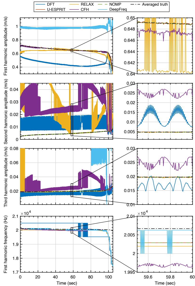
Figure 8: Sinusoidal parameter estimation of the three harmonics' amplitudes and fundamental harmonic's frequency for synthetic signal. The legend shown above applies to all plots.
