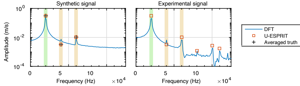
Figure 7: Demonstration of the DFT spectra and Unitary ESPRIT line spectra for the synthetic signal (left) and experimental signal (right). To extract sinusoidal parameters of the first three harmonics: first, a maximum amplitude of the fundamental is searched for, represented by the green shaded area; second, integer multiples (two and three times) of the green shaded area are created and represented by the yellow shaded area; lastly the peak is searched within the yellow shaded area, within a \pm 2/N tolerance.
