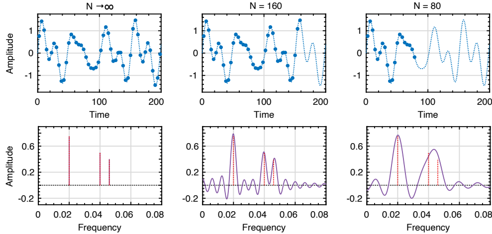
Figure 3: Demonstration of the frequency resolution of a signal with a fixed sampling frequency, with respect to the Rayleigh limit 1/N seen by the DFT, adapted from [19]. A multi-sinusoidal signal (dashed blue line) and its Nyquist-Shannon samples (blue circles) are depicted on the top row. The bottom row shows the DFT's frequency resolution (purple line) and the true line spectra (dashed red line). For a finite N , the DFT's frequency resolution is equal to the convolution between the DFT of the signal and the sinc function.
