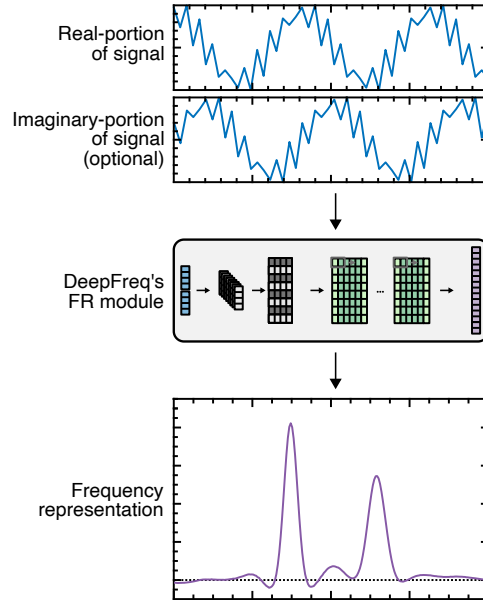
Figure 4: Algorithm flowchart of DeepFreq's frequency representation module. The assumed complex input of the DeepFreq is split into its real and imaginary parts before input. For real-valued signals, the imaginary-valued portion is supplied with zeros of equal length. The frequency representation generates a pseudospectrum (purple line) subject to a peak-picking algorithm.
