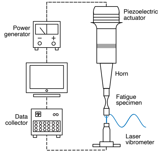
Figure 1: Experimental setup of an ultrasonic fatigue test.
