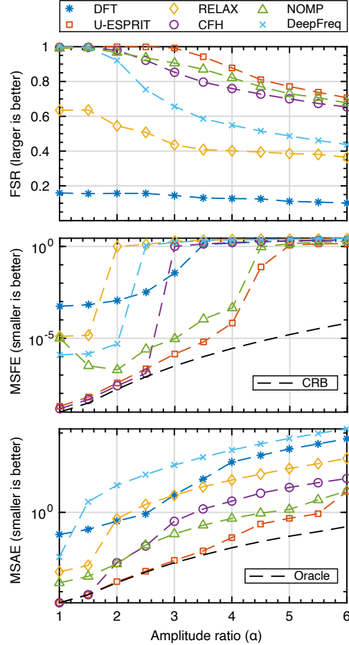
Figure 12: Simulation results for varying amplitude magnitude scaling parameter \alpha . The signal length N = 2^7 , SNR = 40 dB, and model order P = 5 are pre-determined. The legend shown above applies to all plots, with sub-legends within the plots applying only to sub-plots.
