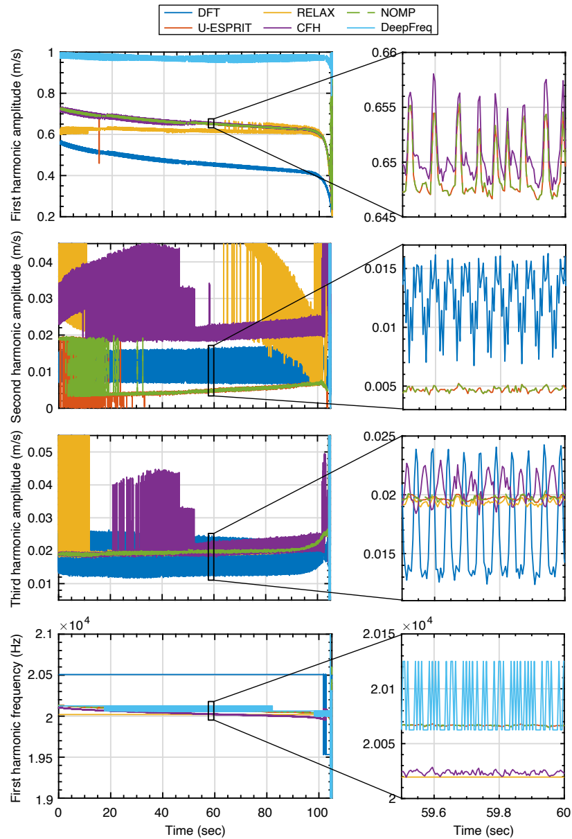
Figure 9: Sinusoidal parameter estimation of the three harmonics' amplitudes and fundamental harmonic's frequency for experimental signal. The legend shown above applies to all plots.
