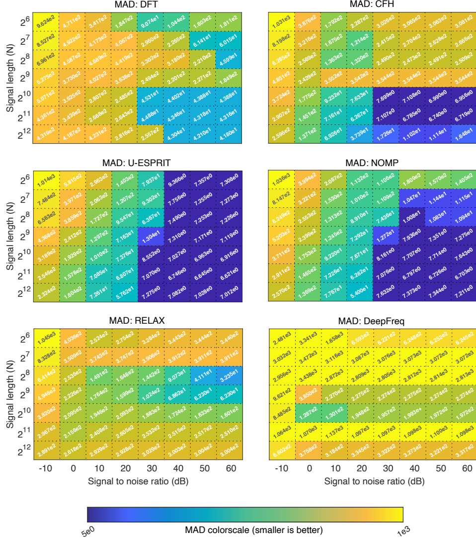
Figure 11: Simulation results as heatmaps of the MAD metric for each LSE, whose colorscales are plotted logarithmically.
