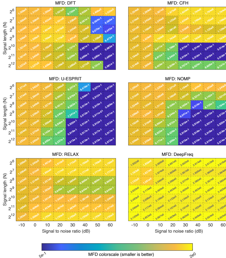
Figure 10: Simulation results as heatmaps of the MFD metric for each LSE, whose colorscales are plotted logarithmically.
