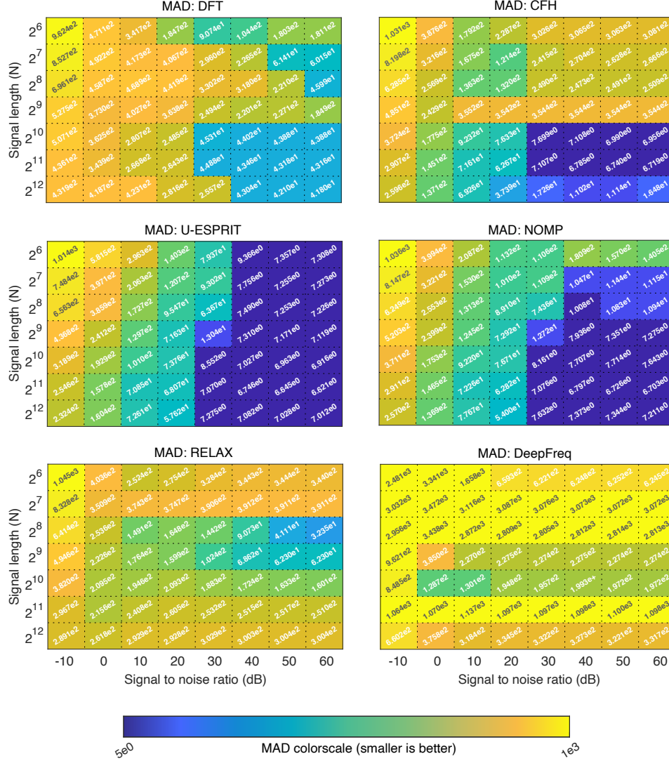
Figure 11: Simulation results as heatmaps of the MAD metric for each LSE, whose colorscales are plotted logarithmically.
