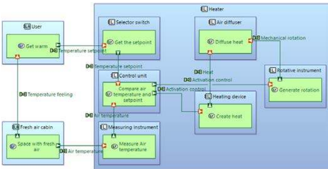
Fig. 17. Results of Logical Architecture diagram
