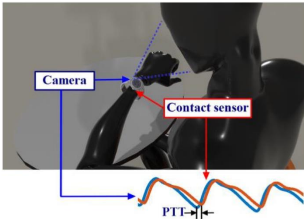
Figure 6. Pulse Transit Time (PTT) corresponds to the time the pulse wave takes to travel from one point of the arterial tree to another. In this example, PTT is computed using PPG waveform analysis of face and wrist. The physiological signals are recorded with a contact sensor (for measuring wrist signal) and a camera (for measuring face signal), both sensors being embedded in a smartwatch. From [39]
