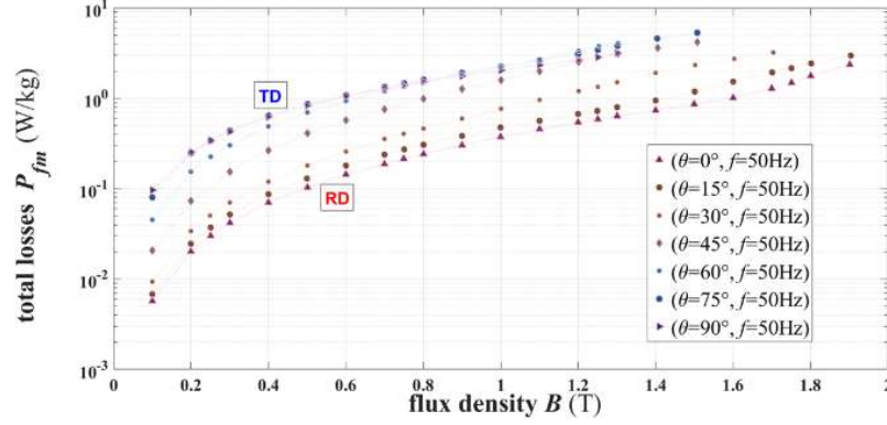
Fig. 8. Total losses P_{fm}(B, \theta) measured on the 7 samples at frequency f = 50 Hz as a function of the magnitude value of flux density B and its angle \theta .
