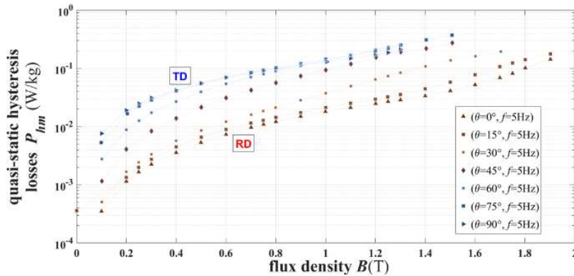
Fig. 7. Hysteresis losses P_{hm}(B, \theta) measured on the 7 samples at low frequency ( f=5\text{Hz} ) as a function of the magnitude value of flux density B and its angle \theta .
