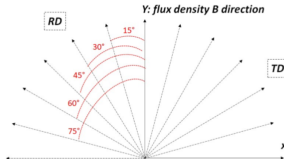
Fig. 5: Definition of cutting angles and flux density directions of specimens.
