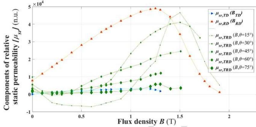
Fig. 9. Components of [\mu_{sr}(B, \theta)] identified as a function of the magnitude value of flux density B for the whole angles \theta ( 0^\circ, 15^\circ, 30^\circ, 45^\circ, 60^\circ, 75^\circ, 90^\circ ).
