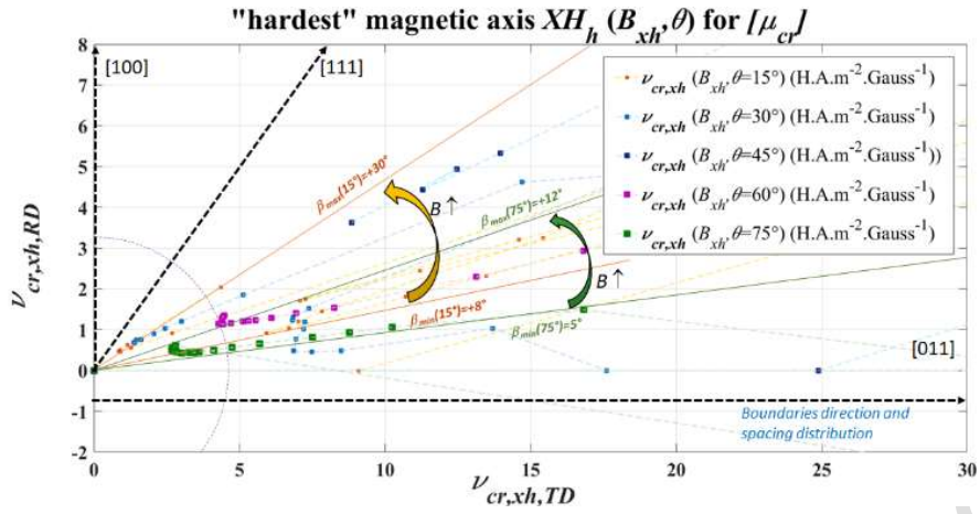
Fig. 15: eigenvectors XH_h and eigenvalues \nu_{c,xh} = \nu_{cr,xh} v_0 with the hardest static coercive field axis of tensor property [v_c] .
