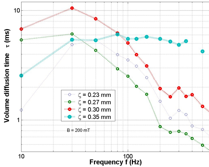
Figure 15: Experimental identification of the volume diffusion time, or the eddy currents time delay, \tau @ 0.2 T.
