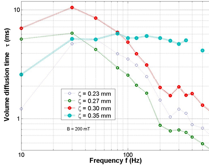
Figure 15: Experimental identification of the volume diffusion time, or the eddy currents time delay, \tau \propto \sigma \mu / K_s @0.2 T.
