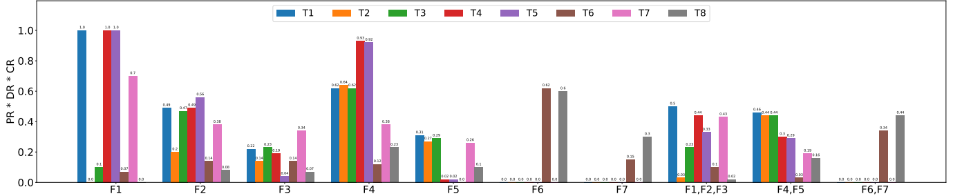
Fig. 1: Comparison of the characterization tests in Table III according to PR * DR * CR , w.r.t to fault models in Table II.
