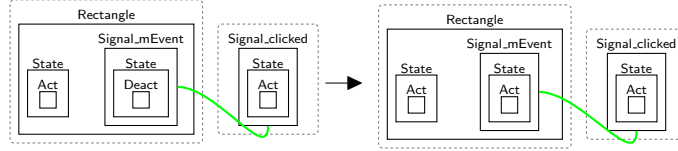
Fig. 6: Activation entity only if parent activated
