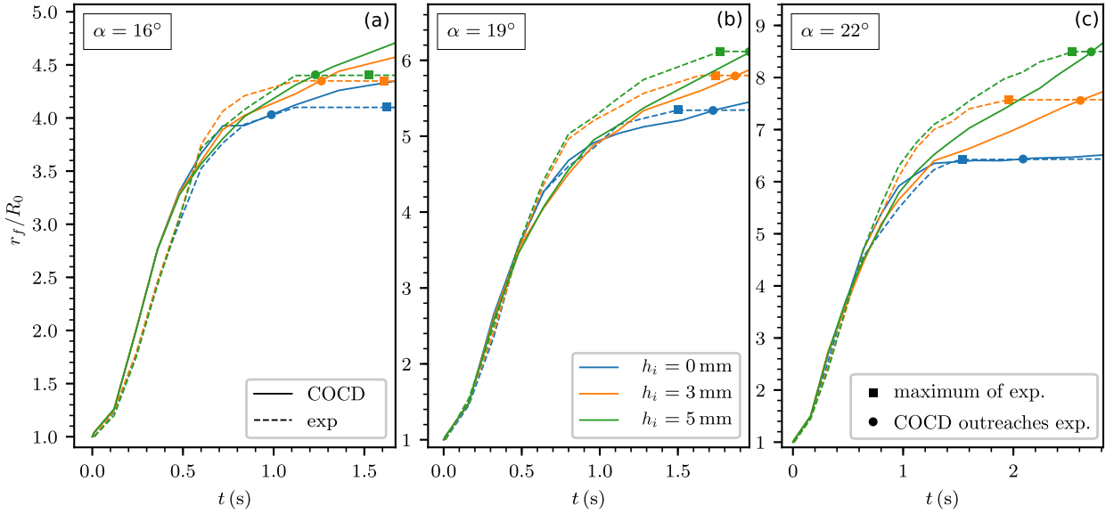
Fig. 9. Evolution of the front position of 2D simulations and experiments. Three inclinations \alpha = 16, 19 , and 22^\circ and three widths of the erodible layer h_i = 0, 3 , and 5 mm are represented. The grain properties are the same in the column and in the erodible layer. In Table A.3, the simulations correspond to rows 1 to 5 and the experiments to row 10. The experiments were carried out by Farini et al. in [61]. Note that the vertical scales differ in Figs. a, b, and c. The squares correspond to the times at which the runout distance is reached in experiments while the circles correspond to the times at which the simulations outdistance the experiments. Note that the final times of simulations are not represented in the figures and that the simulations continue to flow for more than 6 s (see Fig. 11).
