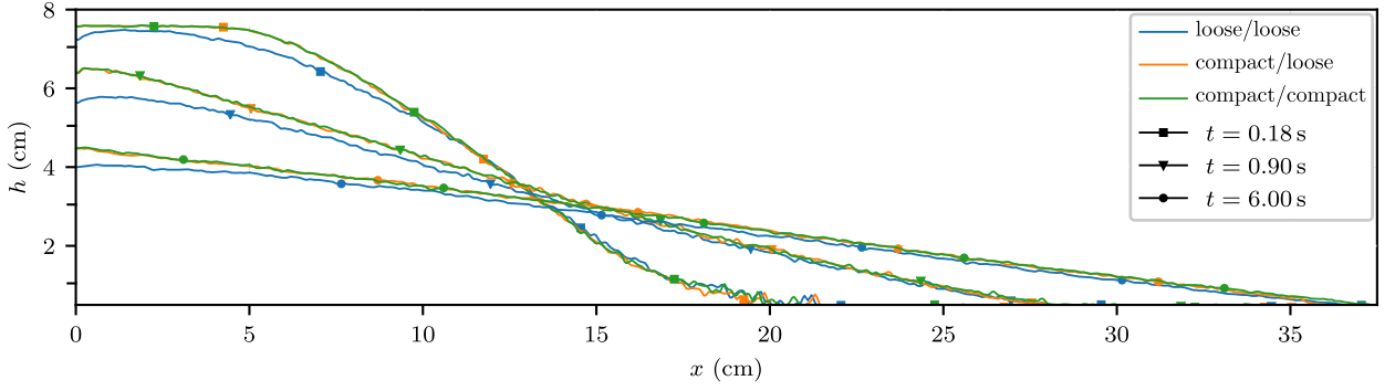
Fig. 18. Profile comparison for different compactions. The slope is \alpha = 22^\circ and the bed thickness is h_i = 5 mm (five grains of mean diameter; see Table A.3, rows 7 to 9). There are no notable differences in front position. However, it can be seen that the maximal height at x = 0 cm is smaller in the loose case. This is probably caused by a compaction of the column during its collapse.
