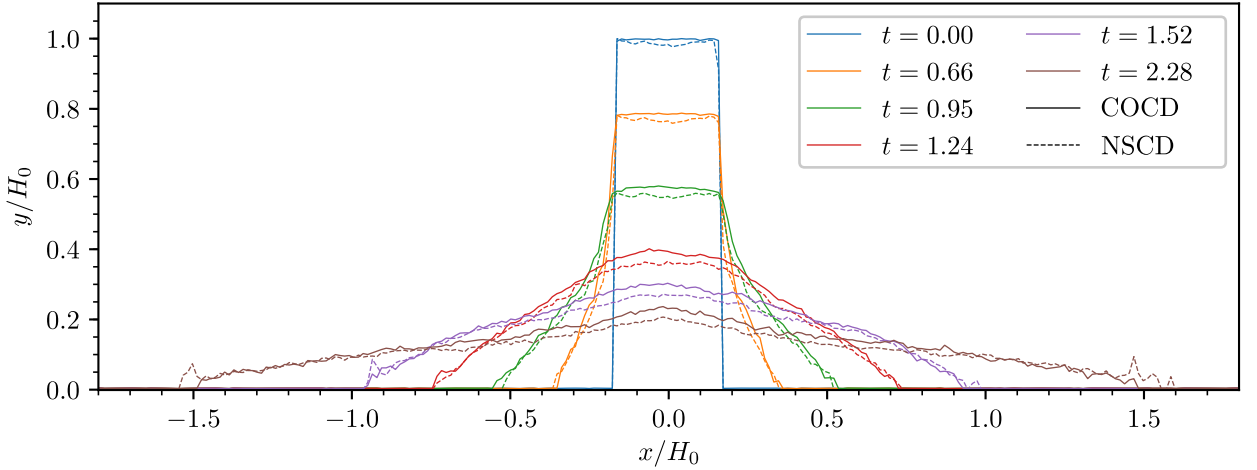
Fig. 4. Comparison of profiles between NSCD and COCD. The reference simulation is a column collapse. In the NSCD simulation [48, 49, 47, 17], there are 6 036 disks and in COCD, N = 7 740 ; see Table A.2, row 3. The plane is horizontal ( \alpha = 0^\circ ). Note that the times given in the legend are normalized by \sqrt{H_0/g} .
