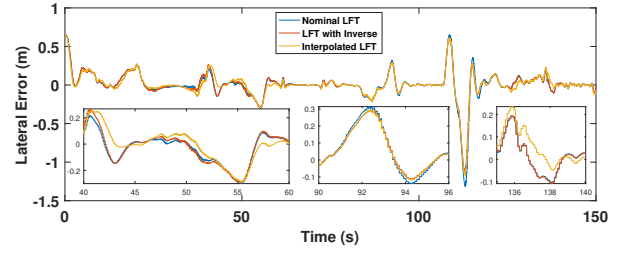
Fig. 12: Lateral error using the LFT approaches ( m )
