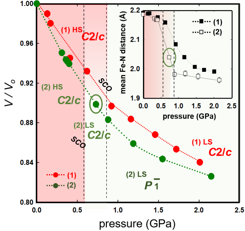
Figure 5. Pressure dependence of the unit cell volume (normalized to the atmospheric pressure volume) for (1) and (2). The inset shows the average Fe-N distances for both compounds. The dotted lines are guides to the eye. The successive spin-state and structural transitions are indicated.
