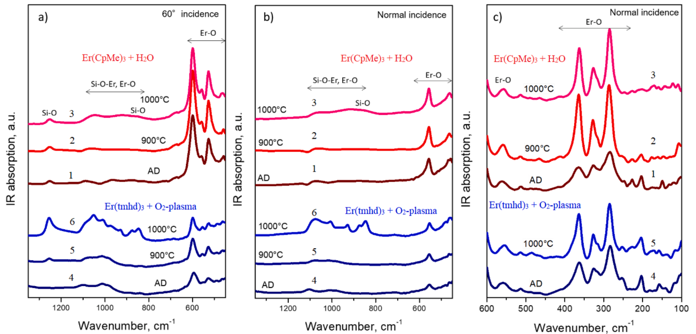
Fig. 8. Comparison of FTIR spectra of as-deposited (AD) and annealed at different temperatures \text{Er}_2\text{O}_3 films grown with \text{Er}(\text{CpMe})_3 by the thermal ALD and with \text{Er}(\text{tmhd})_3 by the plasma assisted ALD. The spectra were recorded with normal and 60^\circ incidence of excitation light and were shifted vertically in the figures for the clarity. Annealing temperatures are mentioned in the figures.
