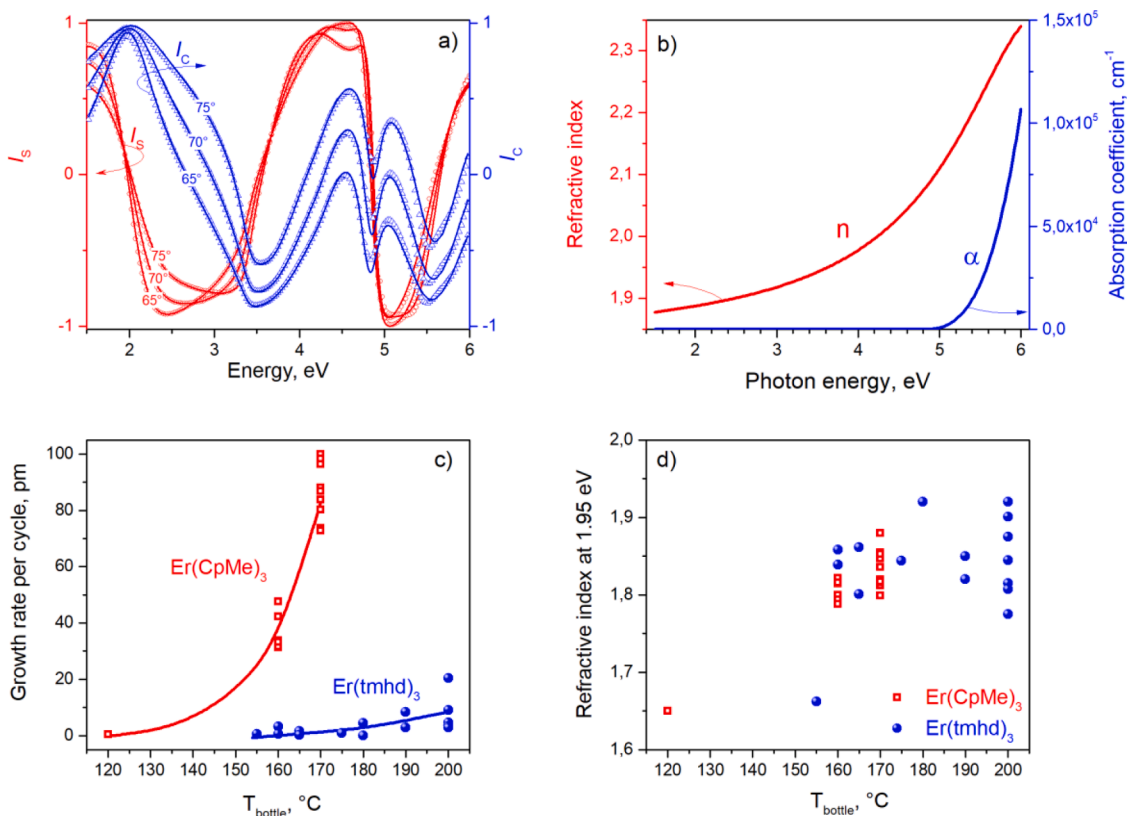
Fig. 2. (a) Typical ellipsometry spectra for as-deposited \text{Er}_2\text{O}_3 film (symbols) taken at 65°, 70° and 75° and their fitting (solid curves) using “new amorphous” model. (b) Refractive index and absorption coefficient of as-deposited \text{Er}_2\text{O}_3 film extracted from the fitting of experimental data in a). (c, d) the effect of bottle temperature on film growth rate per cycle (c) and refractive index (d) for the films deposited with thermal and plasma-assisted approaches using \text{Er}(\text{CpMe})_3 and \text{Er}(\text{tmhd})_3 precursors, respectively. RFP = 2000 W (c, d) for \text{Er}(\text{tmhd})_3 . The different points for the same deposition temperature originate from the different precursor pulse/purge times.
