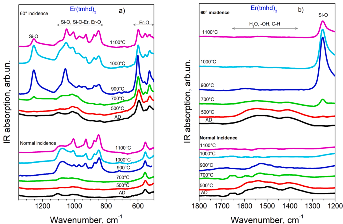
Fig. 7. FTIR spectra of \text{Er}_2\text{O}_3 films grown with plasma assisted ALD versus T_A recorded with normal and 60^\circ incidence of excitation light and presented for different spectral ranges.
