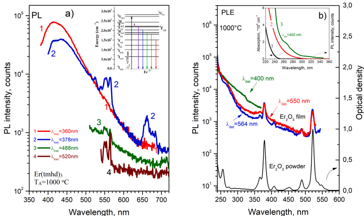
Fig. 14. (a) PL spectra of Er_2O_3 film film prepared with plasma-assisted approach and annealed at 1000 °C. The excitation wavelength is 360 nm (1), 378 nm (2), 488 nm (3) and 520 nm (4); (b) PLE spectra of the same film detected at 400, 550 and 564 nm. The spectrum of optical absorption of Er_2O_3 powder is given for comparison. Inset shows absorption spectra (1,2) and PLE spectrum detected at 400 nm wavelength (3) of the as-deposited film (1) and annealed at 1000 °C (2,3).
