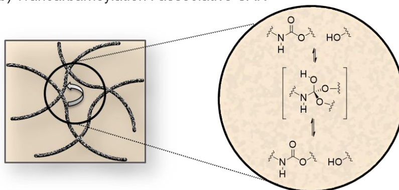
Figure 7. a) Dissociative and b) Associative CANs in polyurethanes chemistry 3.a) Trancarbamylation in PUs networks (urethane/urethane exchange)
