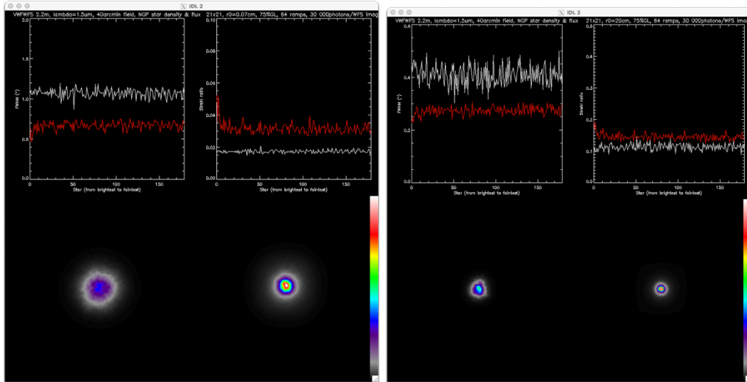
Figure 4(c): same as Figure 4(b) but with NGP star density and fluxes, 180 stars with magnitudes ranging from 10.4 to 18, yielding 30000 photons per WFS image. r_0=0.07\text{m} (left) and r_0=0.2\text{m} (right).
