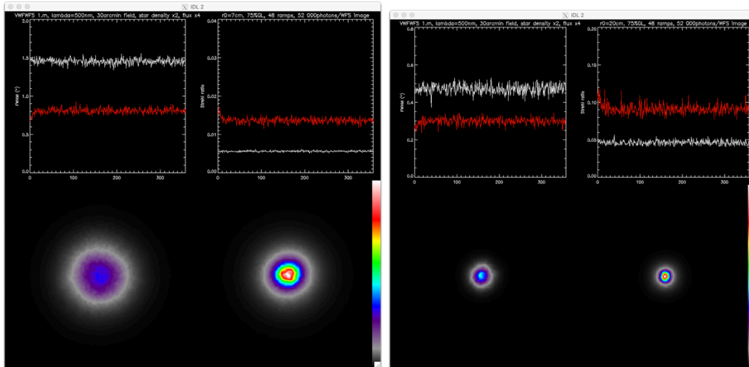
Figure 5(a): 1-m telescope, 11\times 11 DM, r_0=7\text{cm} (left), r_0=20\text{cm} (right) with 75% ground layer turbulence. Field= 30' (star density \text{NGP}\times 4 ), 48 ramps, 52 000 photons per 20\times 20 subimage, 2000 iterations. 500\text{nm} imaging and wavefront sensing wavelength.
