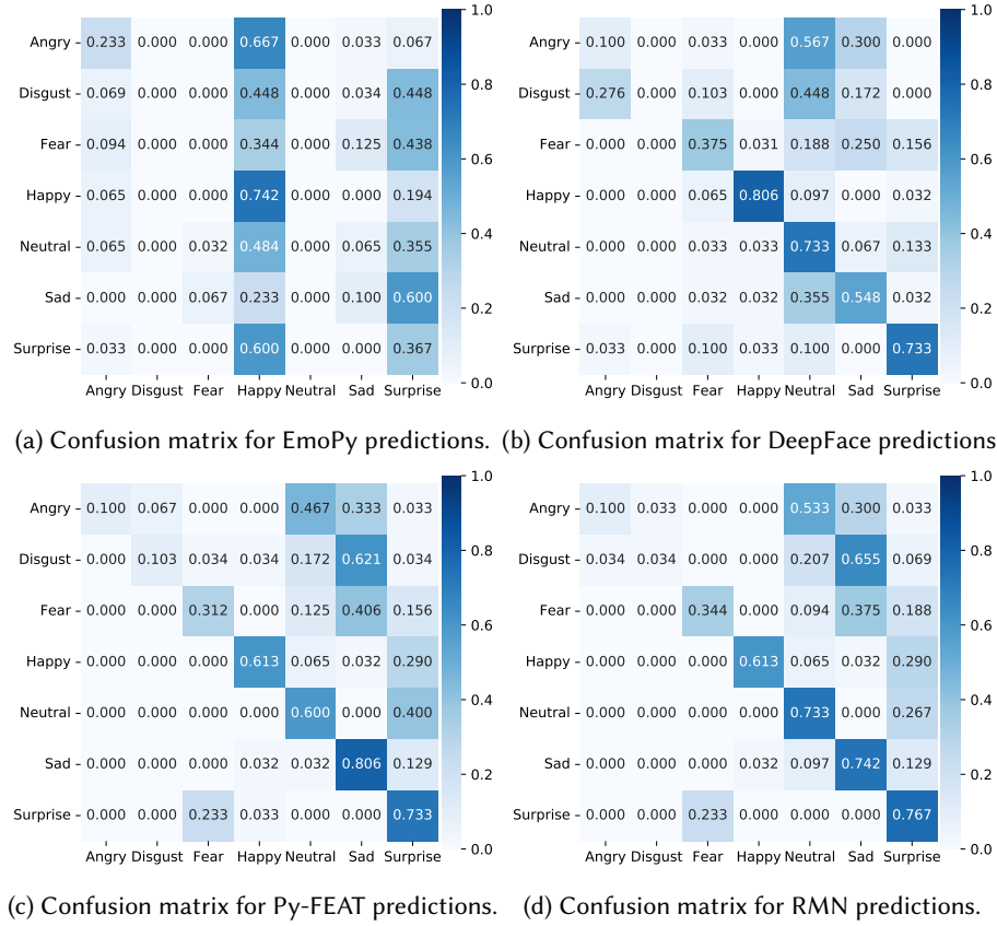
Fig. 6. Illustration of the confusion matrices calculated for the predictions of each library on the JAFFE sample.
