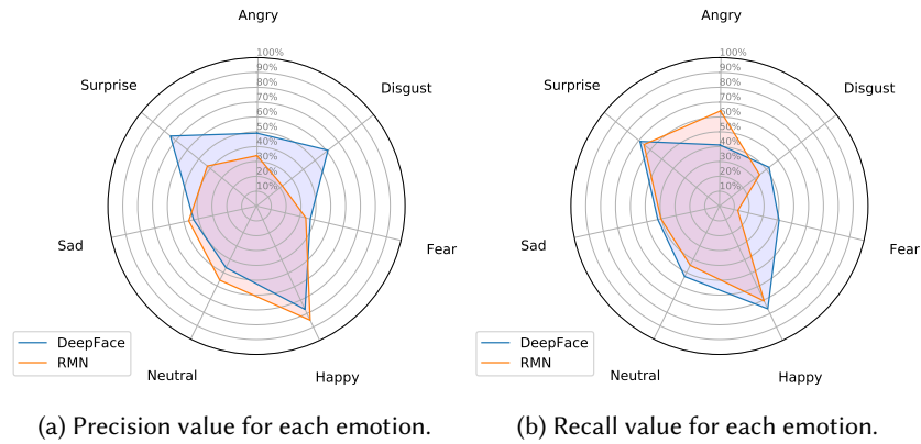
Fig. 9. Illustration of the precision and recall calculated for each emotion on FER-2013 images.
