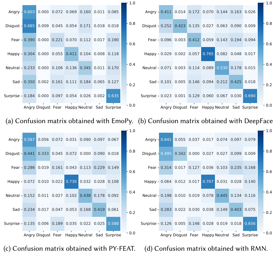
Fig. 8. Illustration of the confusion matrices calculated for the predictions of each library on the FER-2013 sample.
