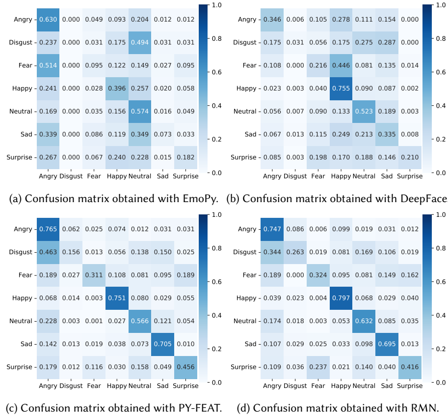
Fig. 10. Illustration of the confusion matrices calculated for the predictions of each library on the RAF-DB sample.
