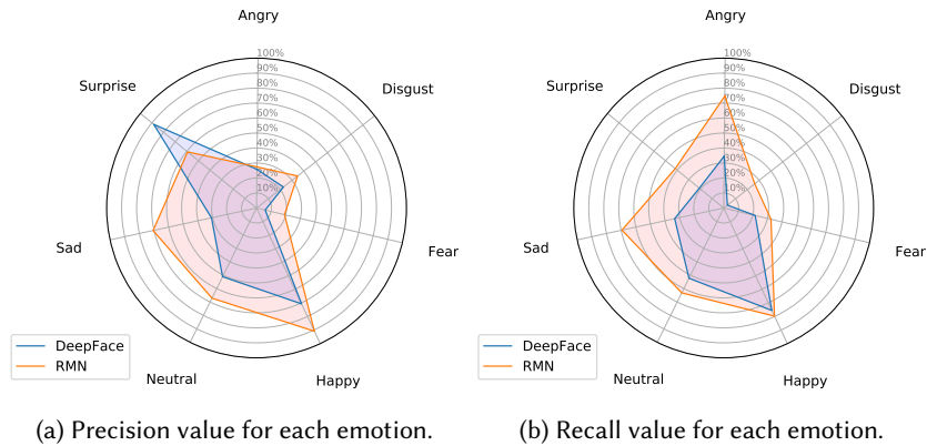
Fig. 11. Illustration of the precision and recall calculated for each emotion on RAF-DB images.
