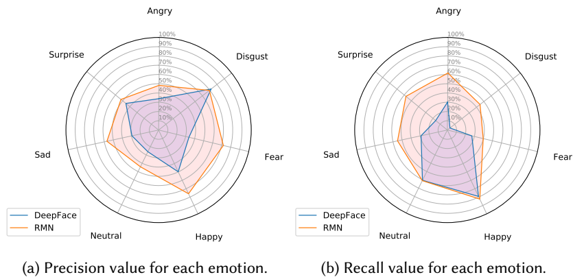
Fig. 13. Illustration of the precision and recall calculated for each emotion on AffectNet images.
