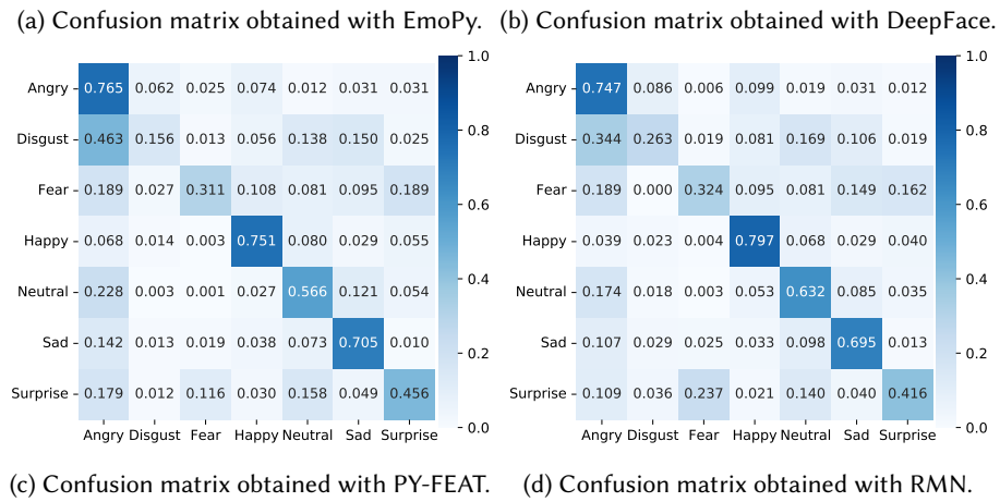
Fig. 10. Illustration of the confusion matrices calculated for the predictions of each library on the RAF-DB sample.
